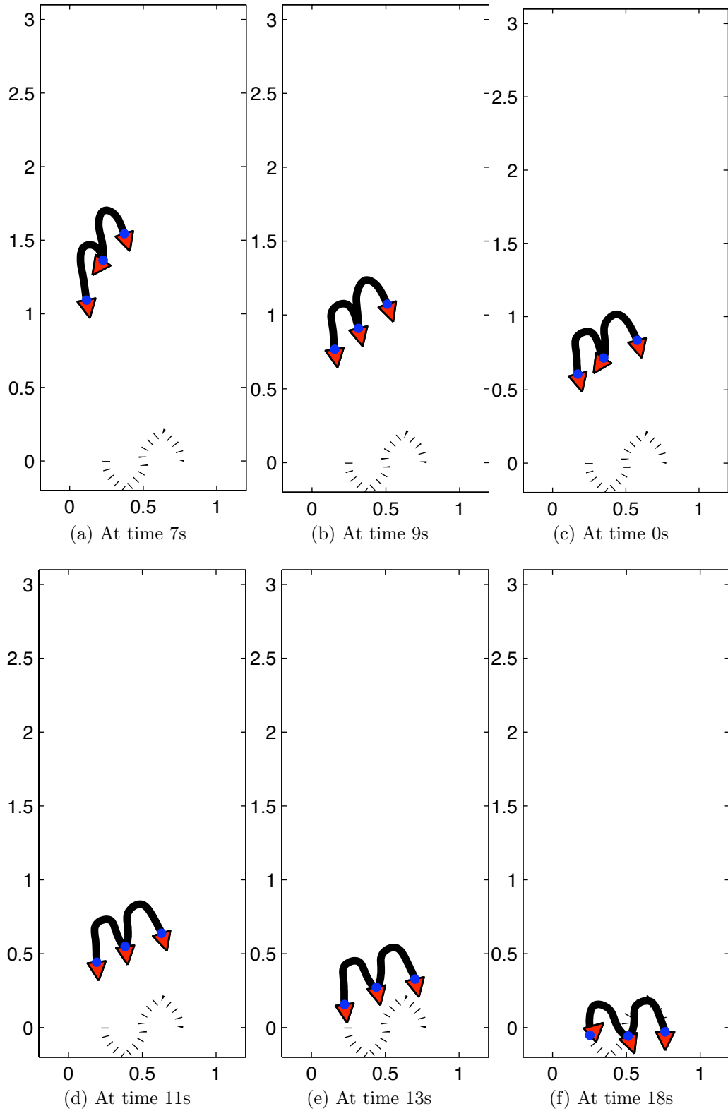
Figure 4.19: Ideal sequence of the hose with hose internal dynamics and dynamic control law(cont.)
