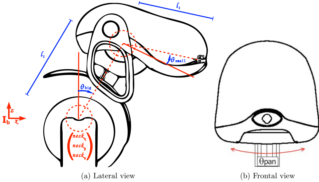
Figure 3.13: Aibo head degrees of freedom
