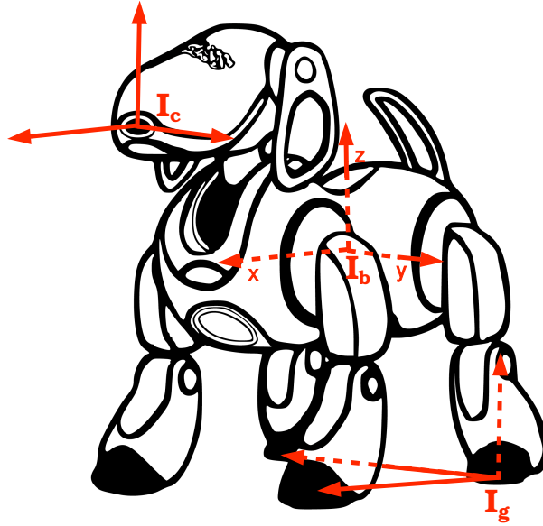
Figure 3.10: Aibo reference systems: I_g, I_b, I_c
