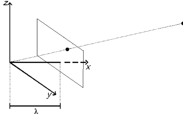
Figure 2.1: Camera reference system and camera projective transformation.
