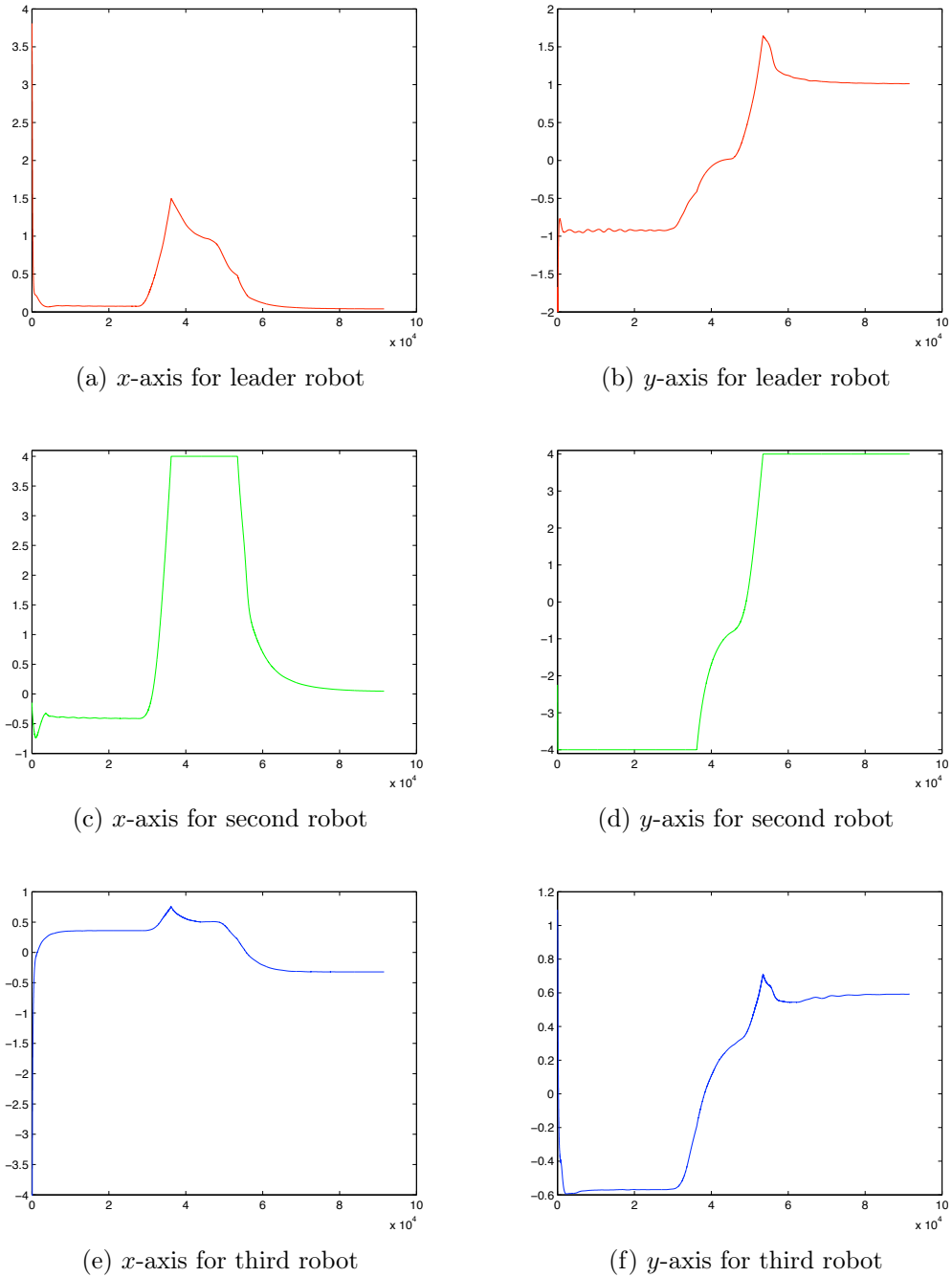
Figure 4.33: Forces applied by robots for the configuration based approach
