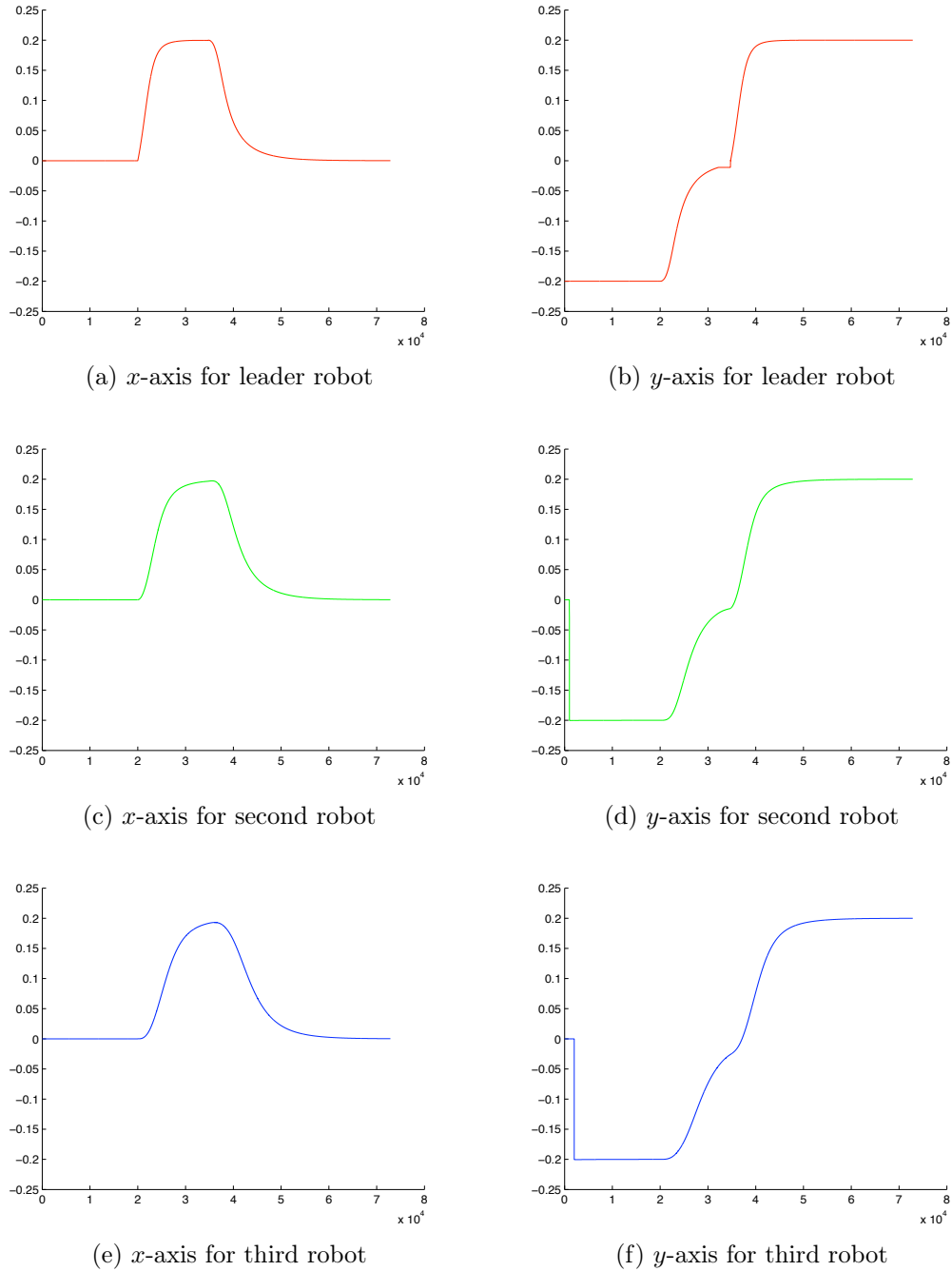
Figure 4.26: Robots velocities during the u-shaped hose transportation for the distance based heuristic f approach.
