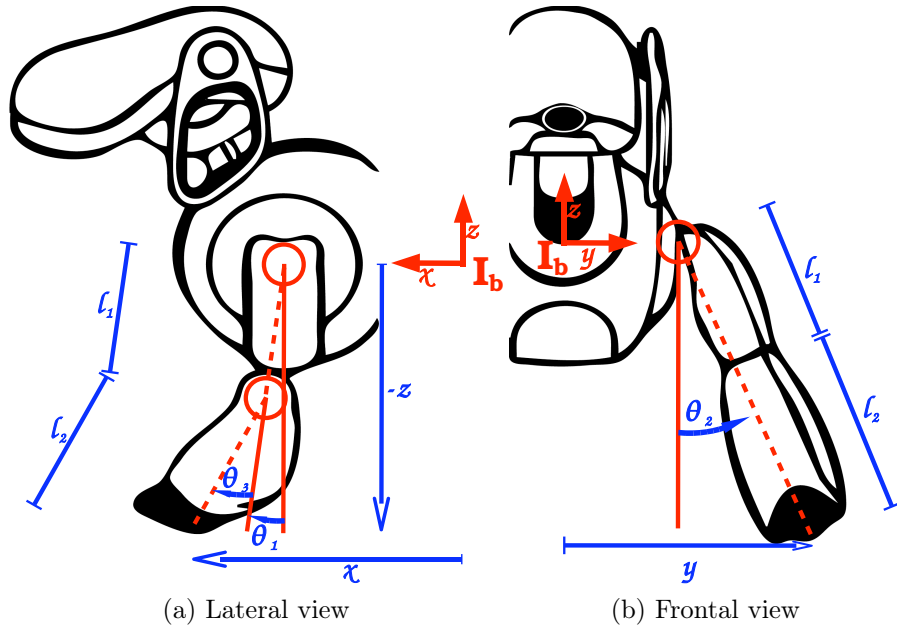
Figure 3.12: Geometry of the leg articulations
