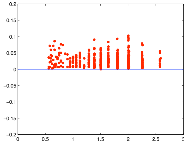
Figure 3.18: Final Visual Servoing error norm distribution versus distance in the 3D world reference system to the ball.
