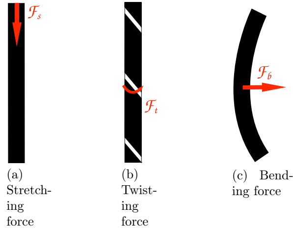
Figure 4.4: Forces induced by the potential energy of the hose
