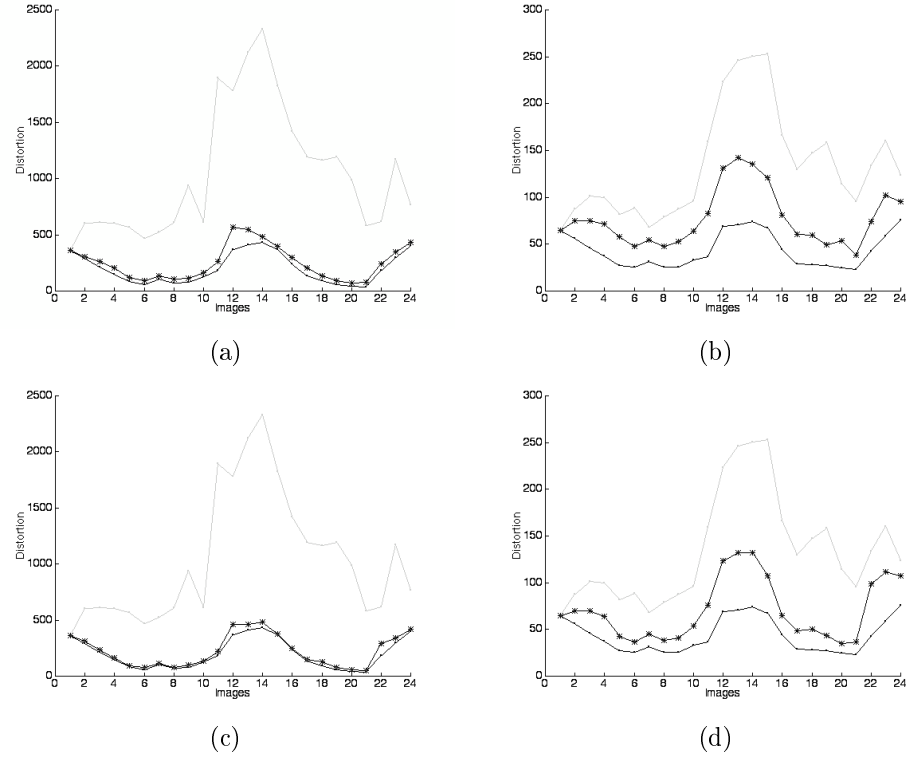
Figure 6.6: Distortion results of the quantization of the full size images in the sequence with the codebooks obtained by the SCL for (a) 16 and (b) 256 color representatives. SCL with penalized distance (equivalent to FSCL) for (c) 16 and (d) 256 color representatives.
