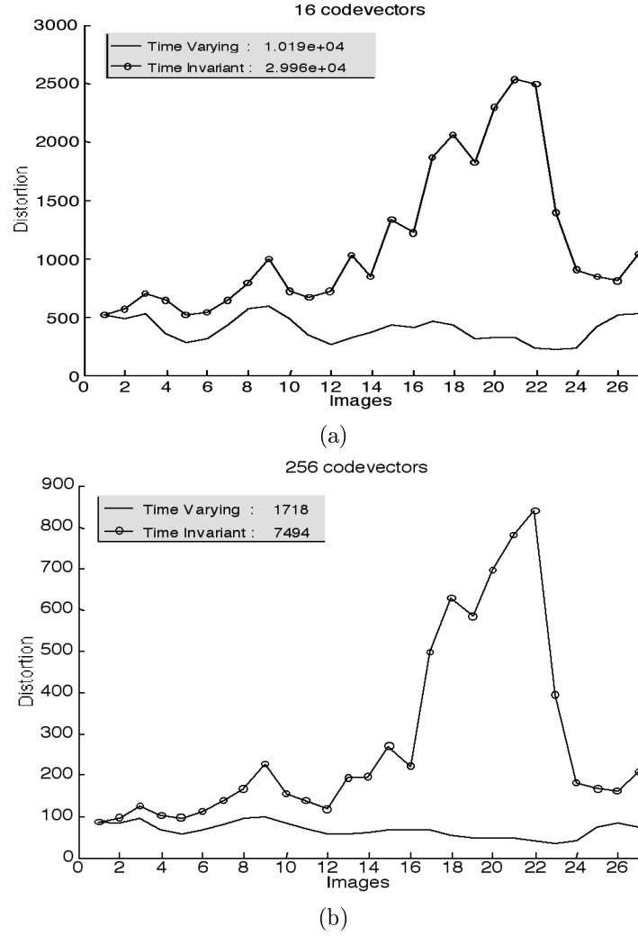
Figure D.13: Reference distortion values obtained with the application of the Time Varying and Time Invariant Heckbert algorithm for (a) 16 colors, (b) 256 colors for sequence2 . The amounts in the legend display the total distortion along the entire sequences.
