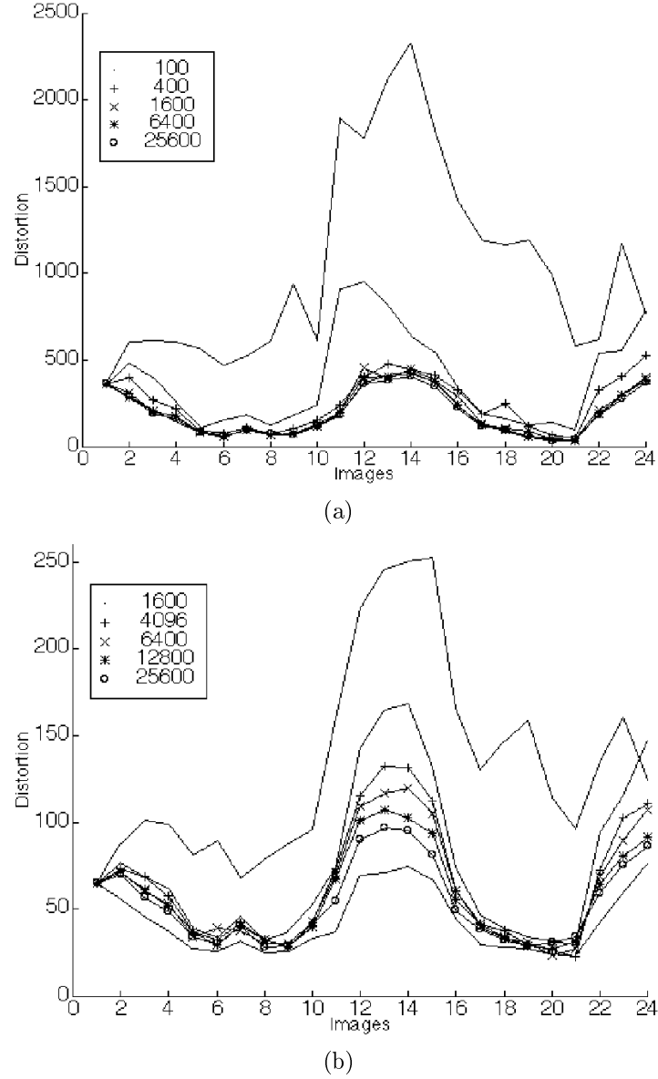
Figure 7.1: Distortion results obtained with the adaptive application of SOM over samples of diverse sizes to compute the color quantizers of (a) 16 (with v_0 = 1 and r = 4 ) and (b) 256 colors (with v_0 = 8 and r = 4 ).
