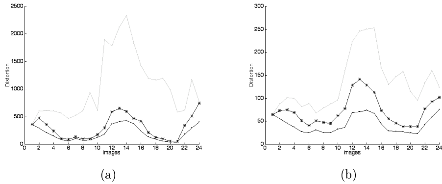
Figure 6.5: Distortion results of the quantization of the full size images in the sequence with the codebooks obtained by the Neural Gas (a) 16 color representatives and (b) 256 color representatives.
