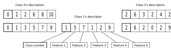
Fig. 5. Examples of classes and their descriptors.
