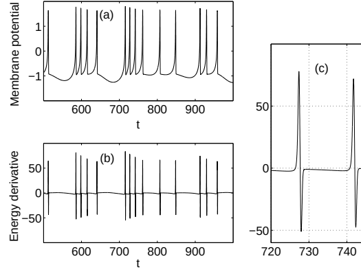
Fig. 2. (a) Action potentials and (b) energy derivative for the Hindmarsh-Rose model neuron. (c) Detail of the energy derivative associated to two action potential spikes showing the energy contributed to the cell to generate the spike (positive area) and the ulterior release of that energy.
