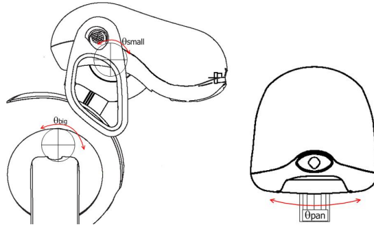
Fig. 5. Geometry of the head articulations
