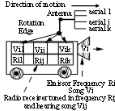
Fig. 1. Agents description.
