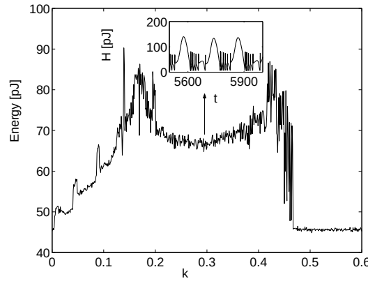
Fig. 4. Energy of one of the two bidirectionally coupled neurons averaged on the attractor at different values of the coupling strength k . In the inset a time series of its energy at k = 0.30 is shown as an example of energy pattern.
