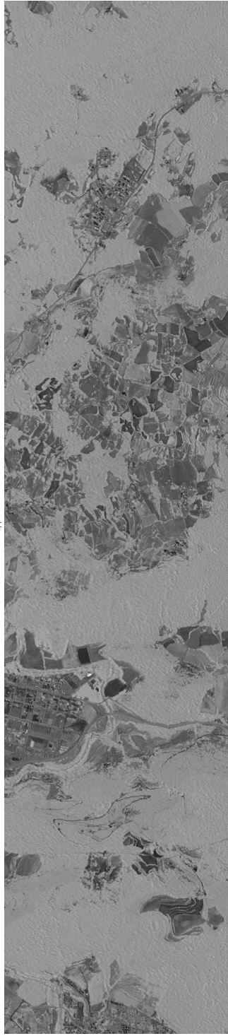
Figure 9.7: Abundance images corresponding to the endmembers discovered by the SIES on the CREAM image (cont.)
