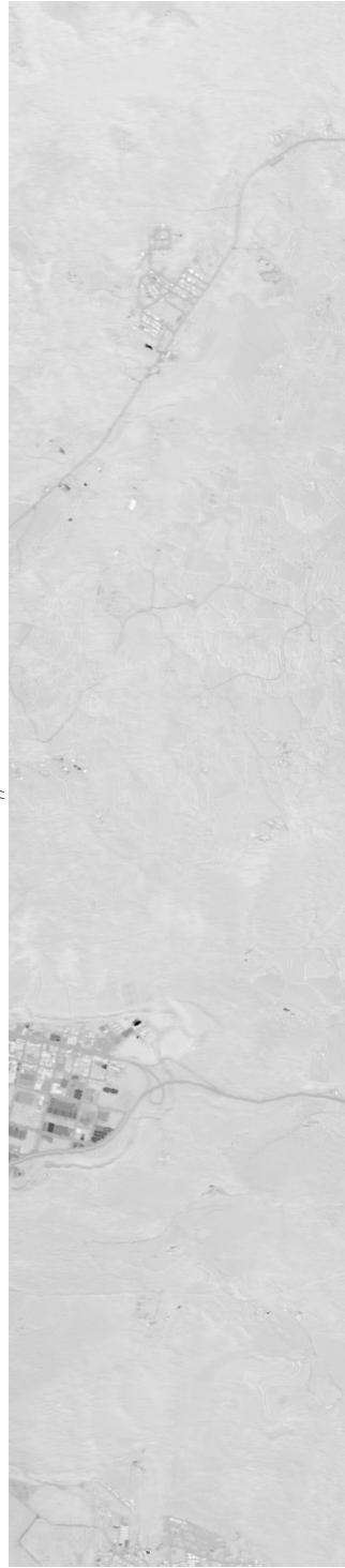
Figure 9.6: Abundance images corresponding to the endmembers discovered by the SIES on the CREAF image
