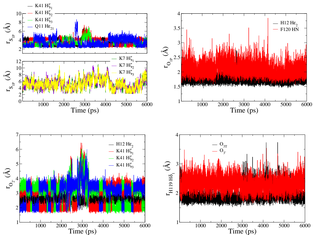
Figure B.10: Time evolution of [\text{S:O}_{\text{IP}}]^{\text{Hyd}} hydrolysis transition state mimic important distances between the ligand and the enzyme residues.
