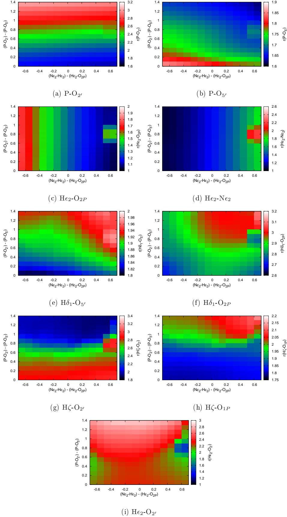
Figure D.3: Some important distances of the QM part of \mathbf{R}_a = (\text{Ne}_2^{\text{His12}} - \text{He}_2^{\text{His12}}) - (\text{He}_2^{\text{His12}} - \text{O}_{2P}) and \mathbf{R}_b = (\text{P} - \text{O}_{2'}) - (\text{P} - \text{O}_{5'}) reaction coordinates in the transphosphorylation step. All distances are in Å.
