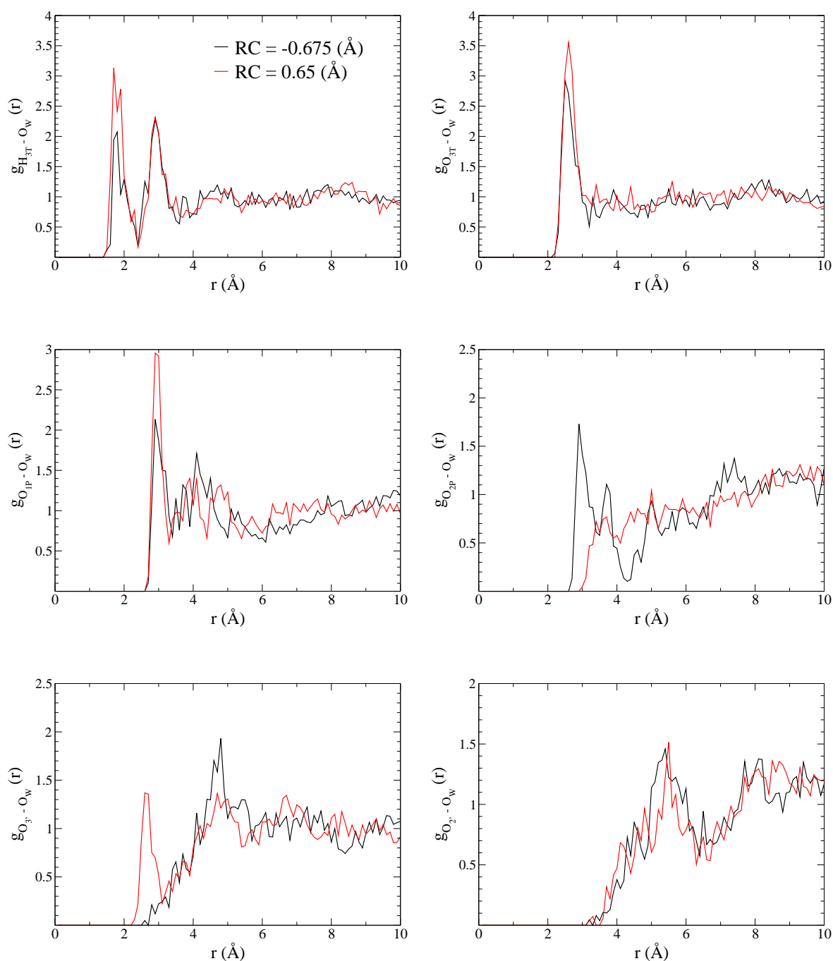
Figure 6.3: Distribution of water around oxyphosphorane's oxygens is shown for two windows of [\text{Hyd}]^{\text{oph}} model, RC = -0.675 Å in black, and RC = 0.65 Å in red. \text{H}_{3T} is at top left corner, at top right corner \text{O}_{3T} is depicted, \text{O}_{1P} and \text{O}_{2P} non-bridging phosphoryl atoms are in the middle left and right, respectively, and finally \text{O}_{3'} and \text{O}_{2'} are at the bottom left and right corner.
