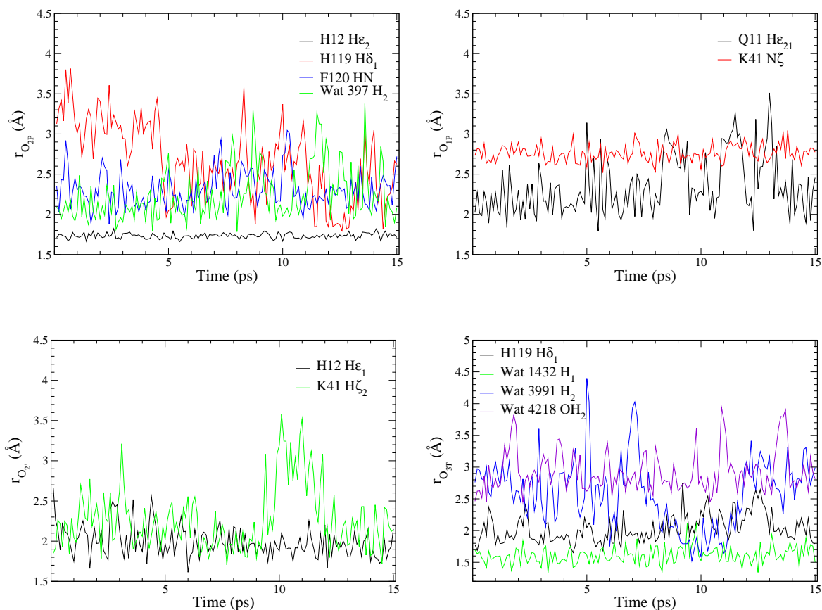
Figure C.3: Dianionic [Hyd] oph model's time evolution of some distances in window centered at reaction coordinate -0.675 Å.
