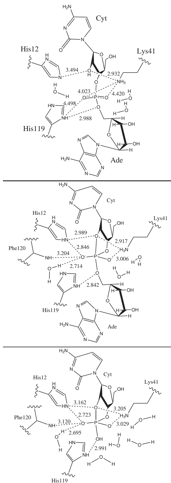
Figure 4.1: Structure of the Reactant model at top, [Trans] TS in the middle and [Hyd] TS at the bottom. Some MD average distances between heavy atoms are depicted.
