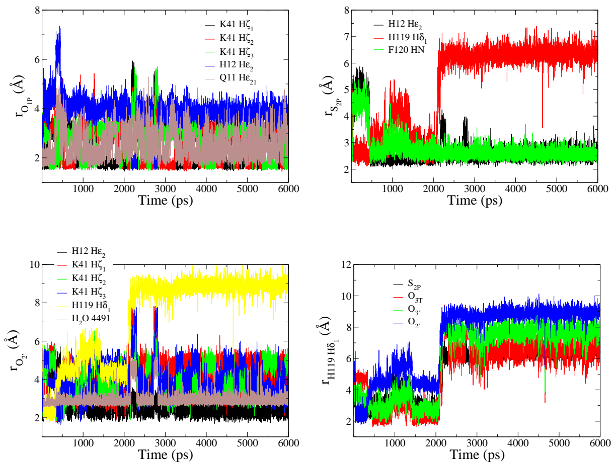
Figure B.11: Time evolution of [S:O_{2P}]^{\text{Hyd}} hydrolysis transition state mimic important distances between the ligand and the enzyme residues.
