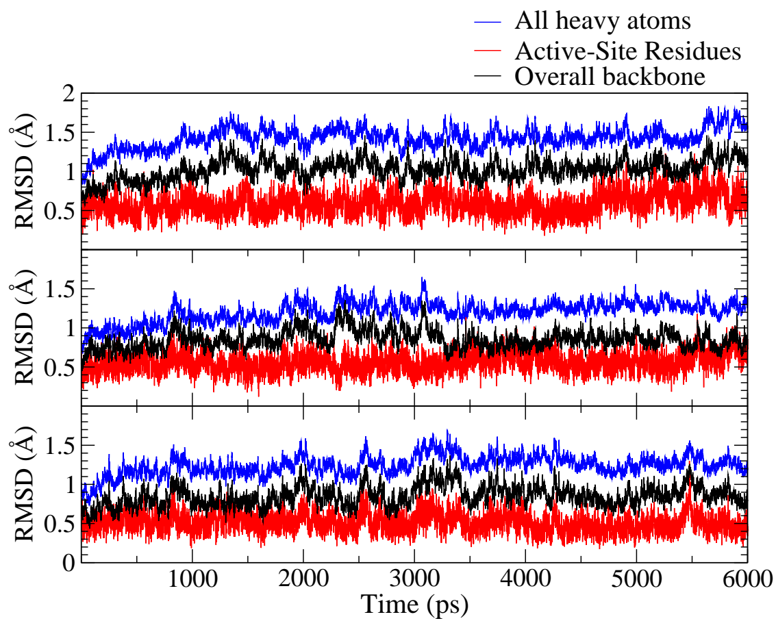
Figure A.1: Root-mean-square deviation of the reactant model at top, the [\text{Trans}]^{TS} mimic model in the middle and the [\text{Hyd}]^{TS} mimic model at the bottom, are represented. On each plot the all-heavy-atom RMSD is shown in blue, the overall backbone in black and the active site residues backbone (His12, His119, Lys41 and the ligand) in red. The RMSD is from the starting conformation overlapping backbone of residues 3 to 122, plotted as a function of the simulation time.
