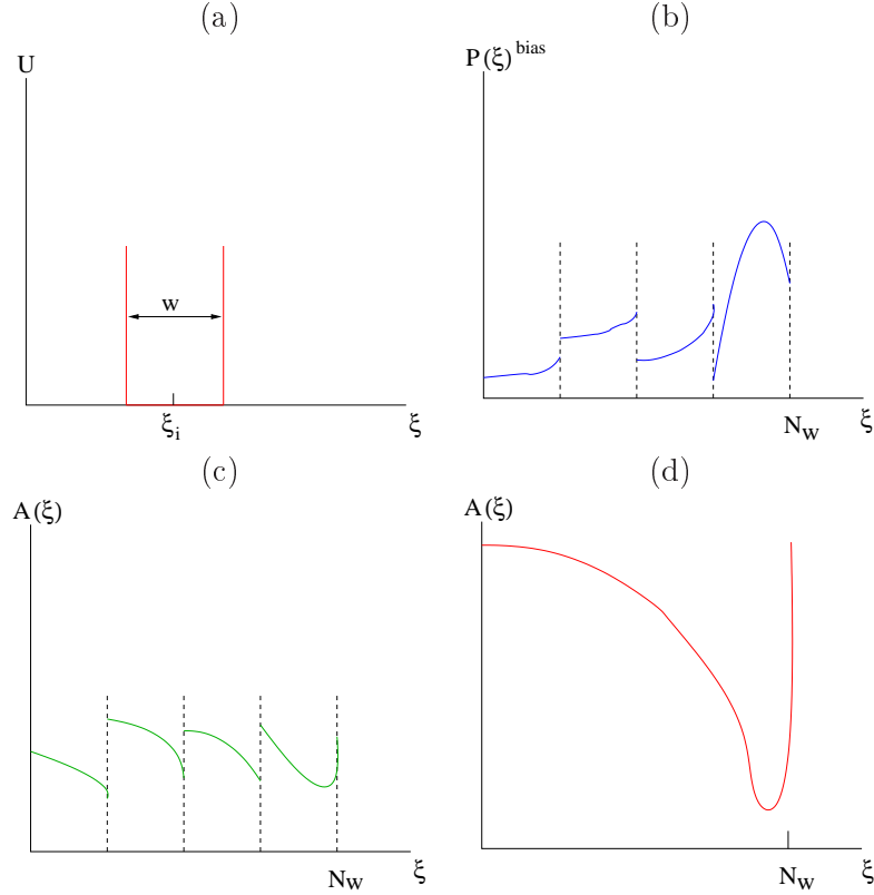
Figure 3.6: Picture (a) shows one of the umbrella potentials, one of the windows. (b) and (c) shows a set of probabilities and Helmholtz free energies, respectively, that would be acquired from each window. Finally, (d) depicted the continuous curve that would be obtained by connecting the A'(q) from each window assuming that umbrellas have points in common with their neighbors.
