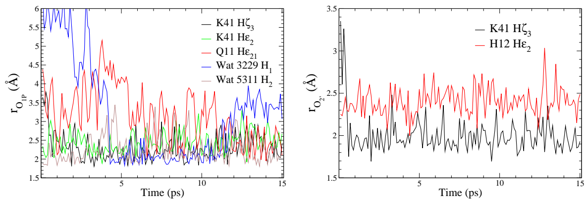
Figure C.4: Dianionic [Hyd] oph model's time evolution of some distances in window centered at reaction coordinate 0.65 Å.
