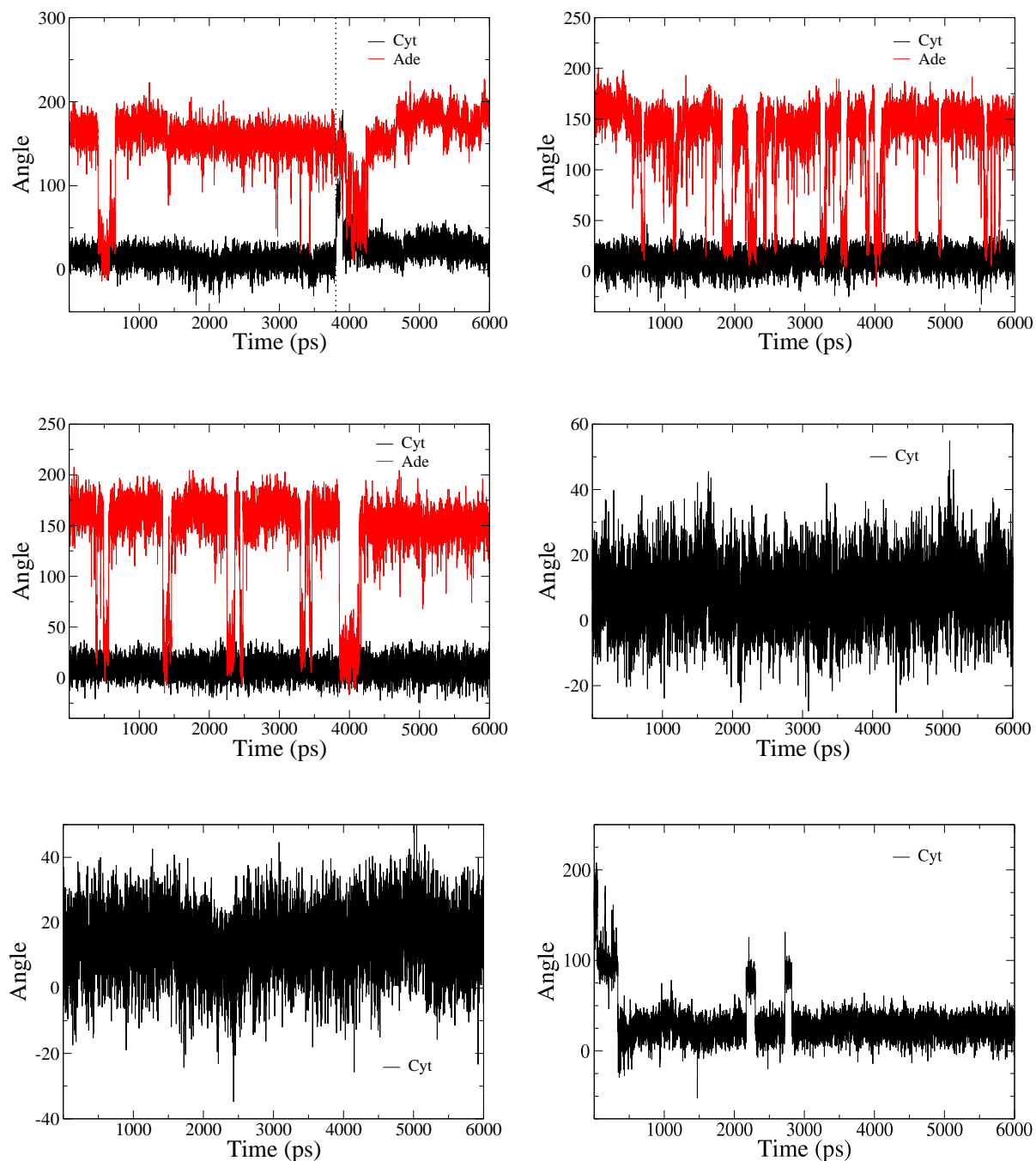
Figure B.3: Phase of all the studied models, plotted as a function of the simulation time. On the first row [S:O_{1P}]^{Trans} and [S:O_{2P}]^{Trans} model's phase are depicted. In the middle, [S:O_{1P},O_{2P}]^{Trans} and [S:O_{1P},O_{2P}]^{Hyd} dithio models are shown. Finally, in the last row [S:O_{1P}]^{Hyd} and [S:O_{2P}]^{Hyd} models are depicted.
