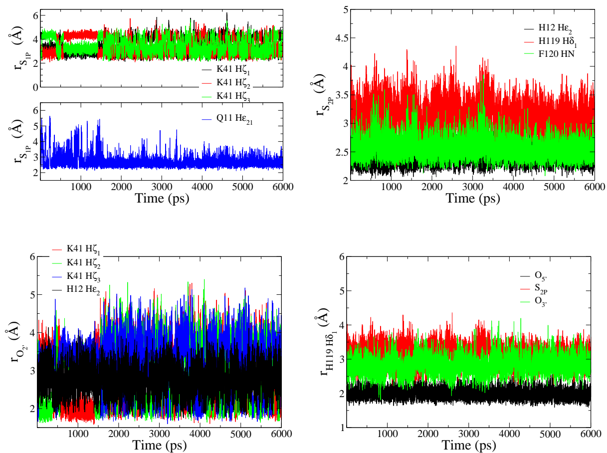
Figure B.8: [\text{S}:\text{O}_{1\text{P}},\text{O}_{2\text{P}}]^{\text{Trans}} transphosphorylation transition state mimic's important distances between the ligand and the enzyme residues, plotted as a function of the simulation time.
