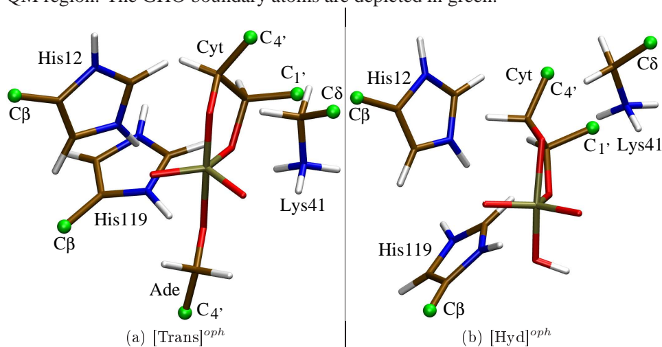
Figure 6.1: a) Representation of the 44 atoms which make up the [\text{Trans}]^{\text{oph}} model QM region. b) Representation of the 41 atoms which make up the [\text{Hyd}]^{\text{oph}} model QM region. The GHQ boundary atoms are depicted in green.
