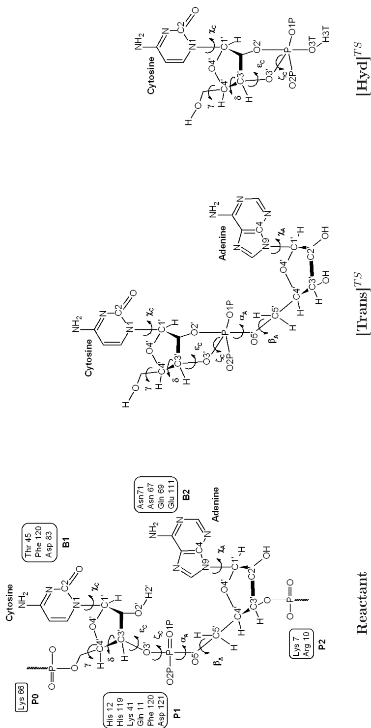
Scheme 4.1: Schematic representation of the RNase A active site with a bound RNA ligand (CpA). The subsites interacting with RNA bases ( B_i ) and phosphate groups ( P_i ) are indicated for the reactant state (left). The transphosphorylation ( [\text{Trans}]^{TS} ) and hydrolysis ( [\text{Hyd}]^{TS} ) transition state mimics are shown in the middle and right, respectively. The atomic names and torsional angles discussed in the text are indicated. [\text{Trans}]^{TS} and [\text{Hyd}]^{TS} are renamed as [\text{native}]^{\text{Hyd}} in Section 5.
