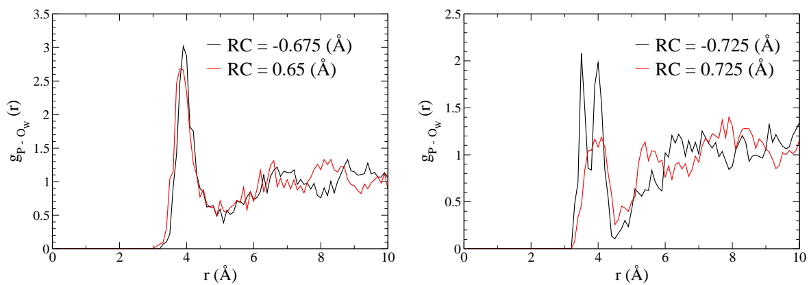
Figure C.7: Distribution of water around phosphorus atom is shown for two windows of [Hyd] oph model in the left hand-side ( RC = -0.675 Å in black, RC = 0.65 Å in red) and for other two windows of [Trans] oph in the right hand-side ( RC = -0.725 Å in black, RC = 0.725 Å in red).
