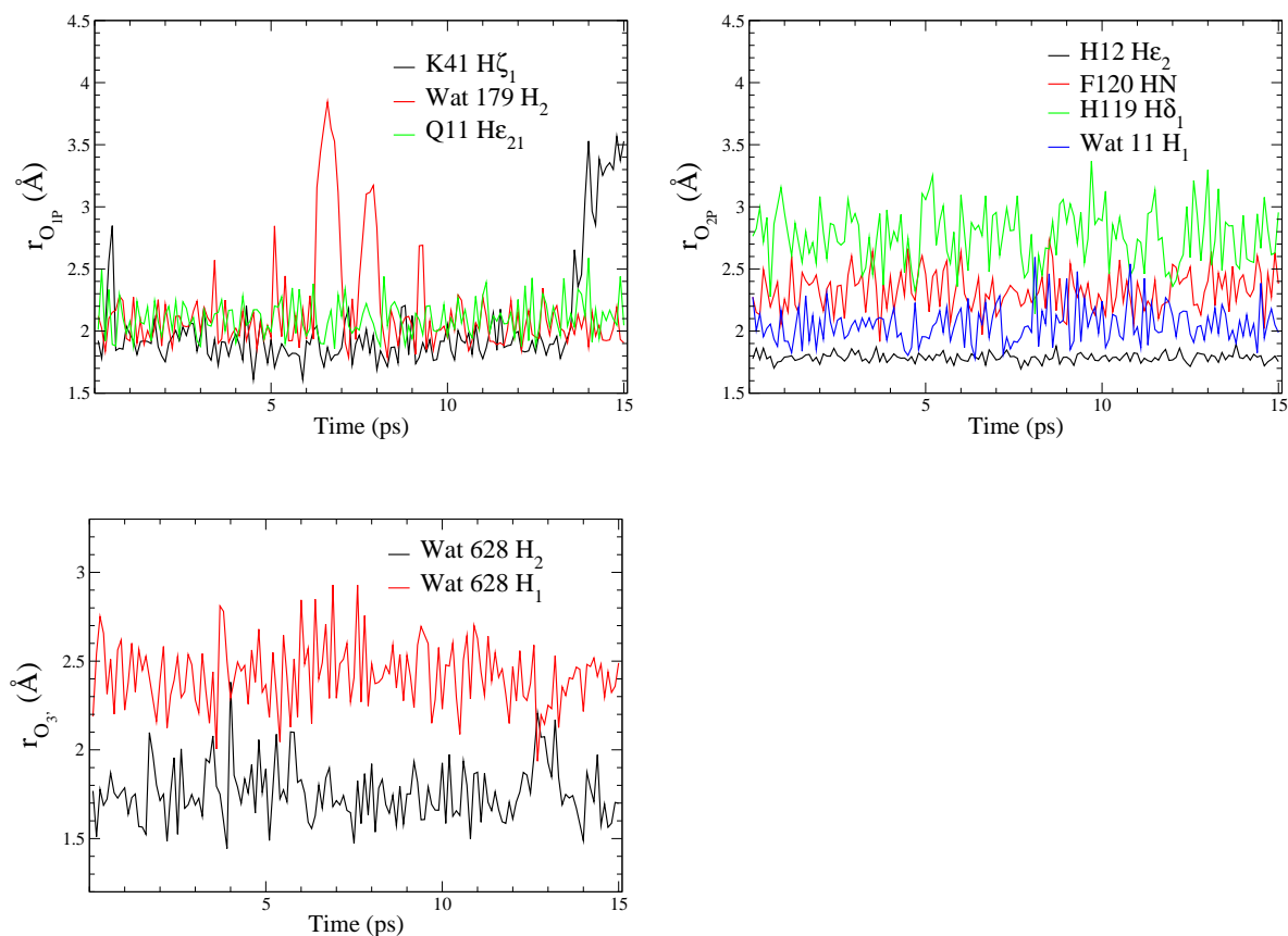
Figure C.6: Monoanionic [Trans] oph model's time evolution of some distances in window centered at reaction coordinate 0.725 Å.
