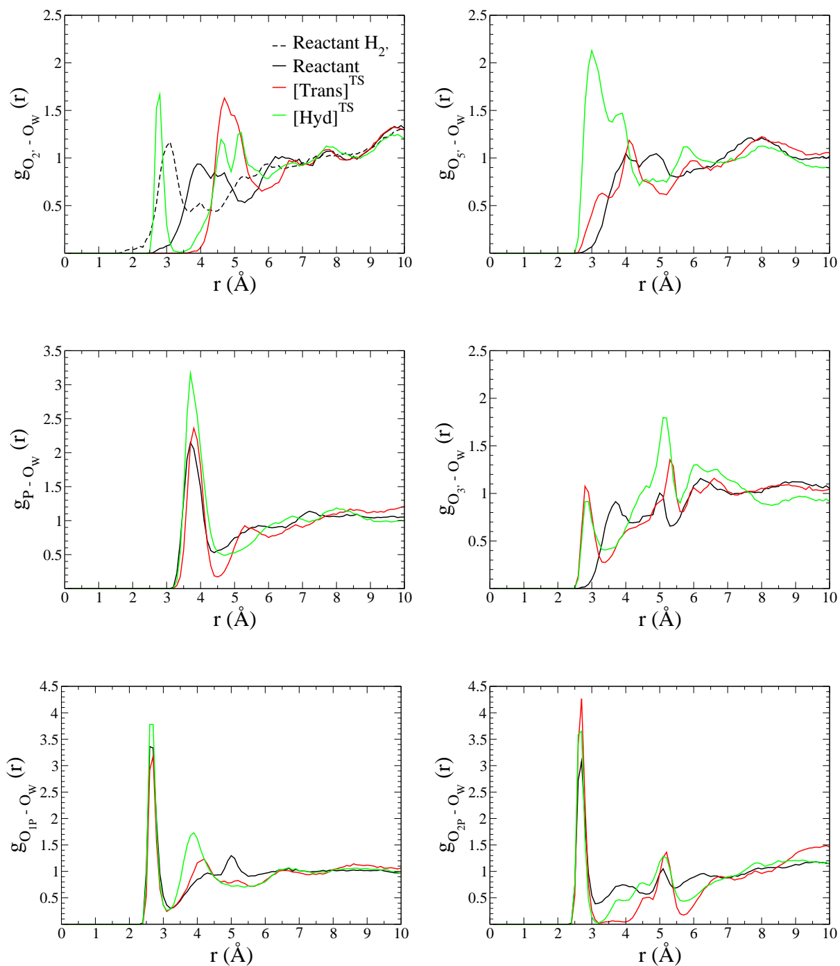
Figure 4.2: Distribution of water around phosphorus atom, phosphate and phosphorane oxygens's atoms is shown for reactant model in black, [\text{Trans}]^{TS} model in red and [\text{Hyd}]^{TS} model in green. \text{O}_{2'} is at top left corner, at top right corner \text{O}_{5'}/\text{O}_{3T} is depicted, phosphorus atom is in the middle left and on the right side is \text{O}_{3'} oxygen, finally \text{O}_{1P} is at the bottom left corner and at the right corner \text{O}_{2P} are shown.
