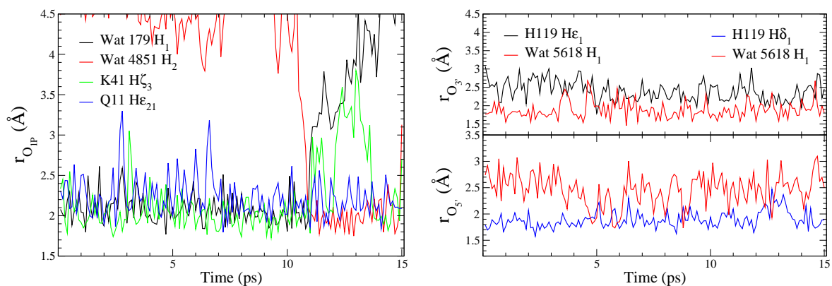
Figure C.6: Monoanionic [Trans] oph model's time evolution of some distances in window centered at reaction coordinate 0.725 Å.
