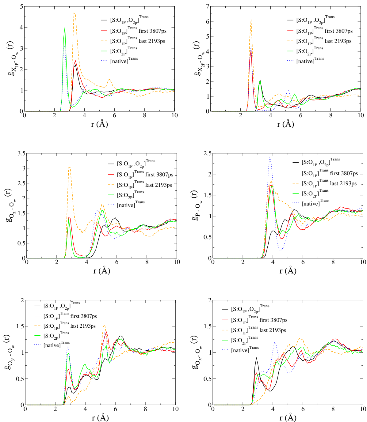
Figure B.4: Radial distribution functions of water oxygens around phosphoryl atoms, for the transphosphorylation transition state mimic thio substituted models. Equatorial phosphoryl atoms are at the top, on the left corner 1P and on the right 2P. At the center O_2' , axial oxygen is on the left and P atom on the right, while at the bottom O_3' , equatorial oxygen is on the left and O_5' , axial oxygen on the right.
