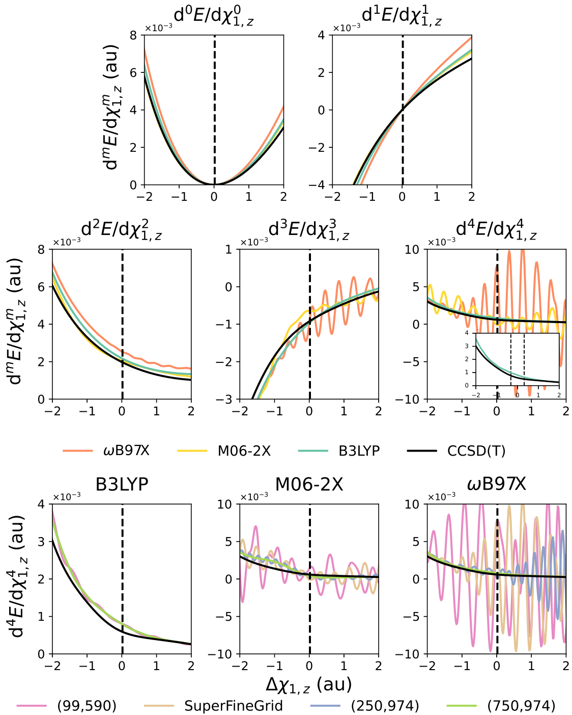
Figure 8.1: Grid-related spurious oscillations affecting the derivatives of the total energy with respect to \chi_{1,z} of HCN · HF, d^mE/d\chi_{1,z}^m ( m = 0 - 4 ). Top and middle row panels show the results of DFAs combined with the (99, 590) grid. In the bottom row panels, curves of d^4E/d\chi_{1,z}^4 obtained with various integration grids are shown. In all plots, the black solid curve represents the CCSD(T) results and the vertical lines mark the equilibrium distance. All properties are given in atomic units.
