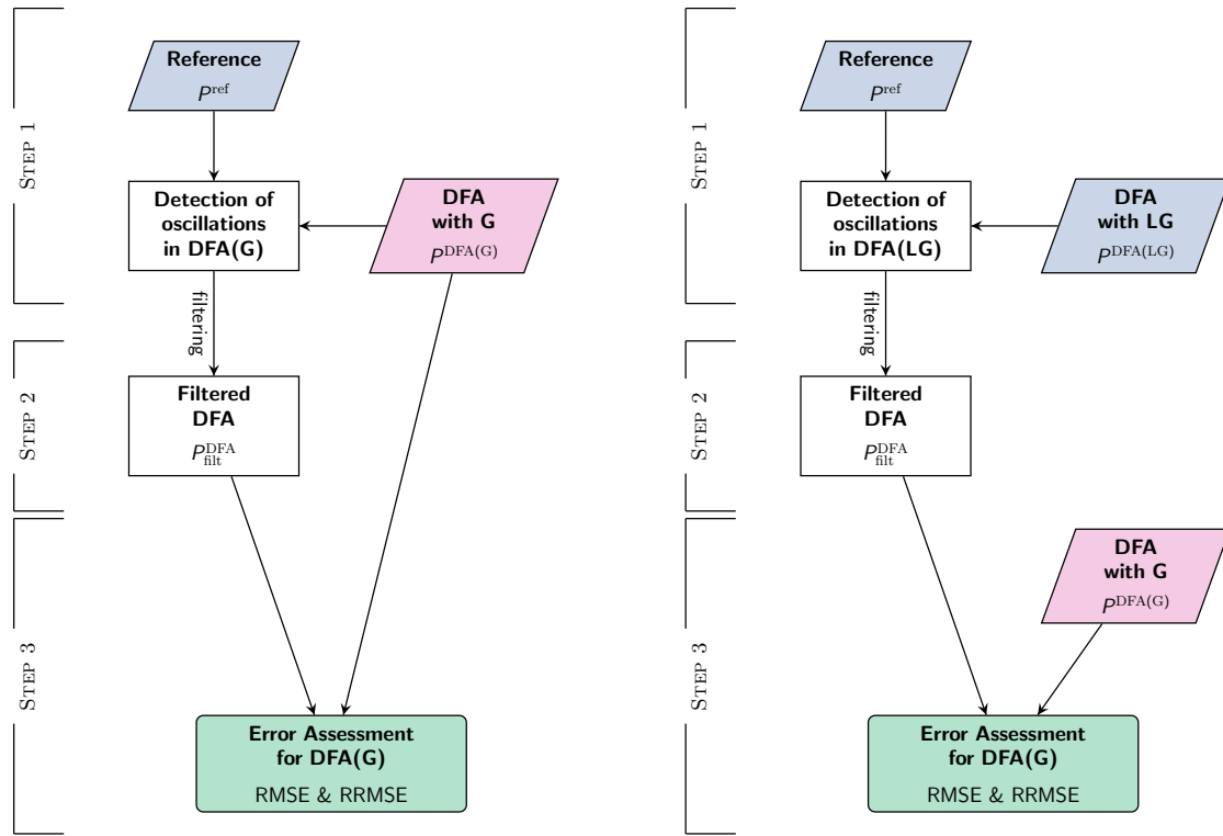
Figure 9.6: Left: Algorithm 1, which tests the property curve obtained with grid G , and also uses this property curve to obtain the filtered curve. Right: Algorithm 2, which uses a larger-grid (LG) to obtain the filtered curve that will be used to quantify the spurious oscillations on a smaller grid ( G ). In all cases, the same DFA and basis are employed.
