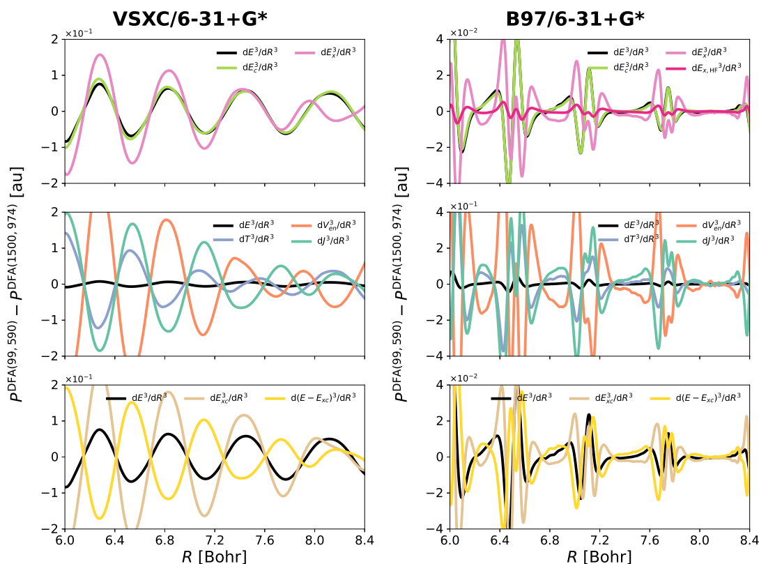
Figure 10.7: Grid-related spurious oscillations in the third derivatives of energy components of \text{Ar}_2 : total electronic ( E ), kinetic ( T ), nuclei attraction ( V_{en} ), Coulomb repulsion ( J ), exact HF-like exchange E_{x,\text{HF}} , exchange ( E_x ), and correlation ( E_c ), as well as their sums. Obtained with VSXC/6-31+G* (left panel) and B97/6-31+G* (right panel) as the difference between (99, 590) and (1500, 974) integration grids.
