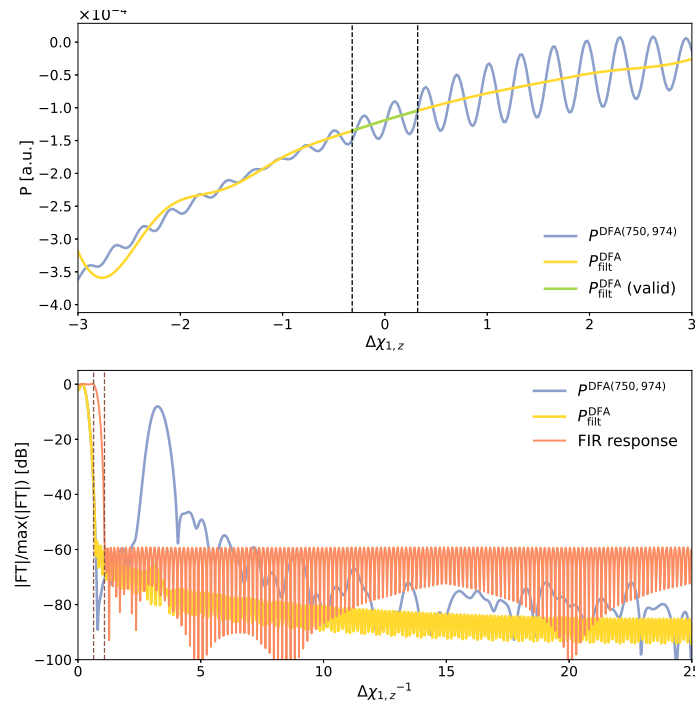
Figure 9.8: Results of the filtering of P^{\text{DFA}(\text{LG})} = P^{\text{DFA}(750,974)} with an automatically designed FIR filter, shown for P = d^3E/d\chi_{1,z}^3 of \text{HCN} \cdot \text{BrH} using \omega\text{B97X/aug-cc-pVTZ} . Top: Original (i.e., unfiltered) and filtered curves in the \chi_{1,z} domain. One can observe the effect of the initial conditions in the left part of the yellow curve. The valid part of the filtered curve within the \{\xi_0\} studied range, is shown in green color. Bottom: Frequency spectra of the original and filtered curve (in reciprocal domain), along with the response of the designed FIR filter (orange, shown in the normalized decibel scale). In the top plot, dashed black vertical lines mark the displacement range of the property curve \{\xi_0\} , for which RMS, RMSE, and RRMSE are calculated. In the bottom plot, dashed orange vertical lines mark the transition band of the designed low-pass filter.
