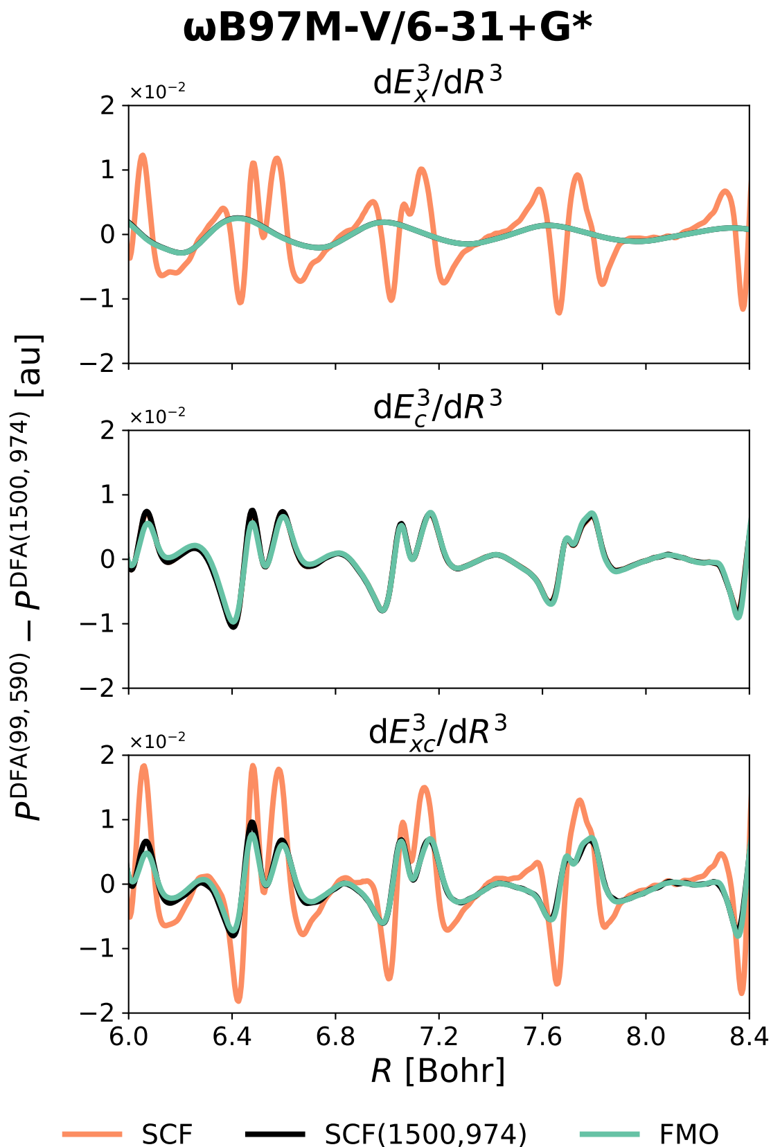
Figure A2.16: Grid-related spurious oscillations in the third derivatives of exchange ( E_x ), correlation ( E_c ) energy components of \text{Ar}_2 , as well as their sum, obtained using \omega B97M-V/6-31+G* and the (99, 590) and (1500, 974) integration grids. Three different types of the input densities are employed: SCF — density obtained in SCF using corresponding grids, SCF(1500, 974) — density obtained in SCF using the reference (1500, 974) grid, FMO — trial density constructed using FMOs obtained for one geometry ( R=7.2 Bohr) and the (250, 974) integration grid.
