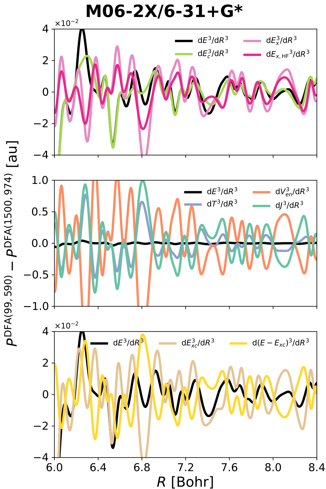
Figure A2.13: Grid-related spurious oscillations in the third derivatives of energy components of \text{Ar}_2 : total electronic ( E ), kinetic ( T ), nuclei attraction ( V_{en} ), Coulomb repulsion ( J ), exact HF-like exchange E_{x,\text{HF}} , exchange ( E_x ), and correlation ( E_c ), as well as their sums. Obtained with M06-2X/6-31+G* as the difference between (99, 590) and (1500, 974) integration grids.
