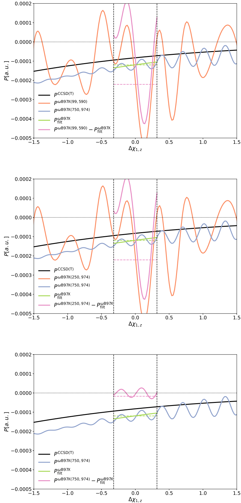
Figure 9.10: The P^{\text{DFA(G)}} , P^{\text{DFA(LG)}} and P^{\text{DFA}}_{\text{filt}} curves of d^3E/d\chi_{1,z}^3 of the HCN·BrH system. Calculated with \omega B97X/aug-cc-pVTZ and three tested grids G = (99, 590) (top), with \text{RMSE} = 2.21 \cdot 10^{-4} and \text{RRMSE} = 184.7\% ; (250, 974) (middle), with \text{RMSE} = 1.51 \cdot 10^{-4} and \text{RRMSE} = 126.3\% ; (750, 974) (bottom), with \text{RMSE} = 1.72 \cdot 10^{-5} and \text{RRMSE} = 14.4\% . In all computations, LG = (750, 974) was utilized. Dashed colored horizontal lines mark the negative value of RMSE (pink) and RMS of the filtered profile (green). Dashed black vertical lines mark the studied range of the property curve \{\xi_0\} , for which RMS, RMSE, and RRMSE are calculated.
