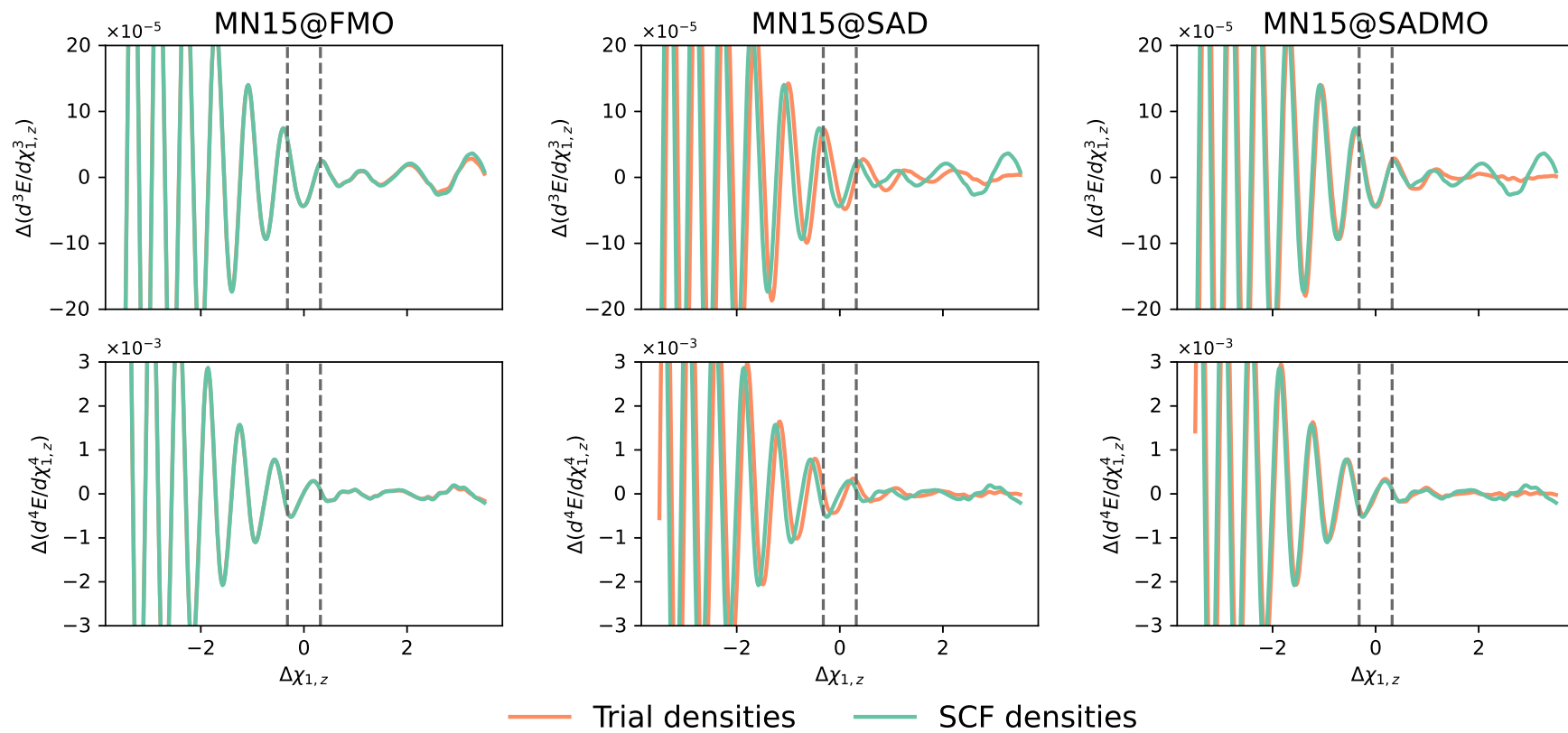
Figure A2.7: Spurious oscillations in d^3E/d\chi_{1,z}^3 and d^4E/d\chi_{1,z}^4 of the \text{HCN} \cdot \text{HF} system, defined as \Delta P = P^{\text{DFA}(99,590)} - P^{\text{DFA}(1500,974)} , obtained with MN15/6-31+G* and the trial densities (orange curves) and the SCF density (green curves, shown on each plot).
