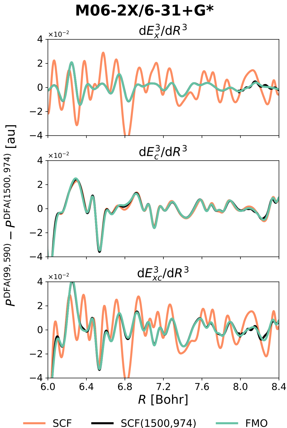
Figure A2.17: Grid-related spurious oscillations in the third derivatives of exchange ( E_x ), correlation ( E_c ) energy components of \text{Ar}_2 , as well as their sum, obtained using M06-2X/6-31+G* and the (99, 590) and (1500, 974) integration grids. Three different types of the input densities are employed: SCF — density obtained in SCF using corresponding grids, SCF(1500, 974) — density obtained in SCF using the reference (1500, 974) grid, FMO — trial density constructed using FMOs obtained for one geometry ( R=7.2 Bohr) and the (250, 974) integration grid.
