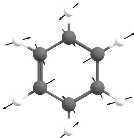
Figure A4.24: Graphical representation of the Q_4 ( E_{2g} ) normal mode of benzene. Obtained at the M06-2X/aug-cc-pVDZ level of theory.
