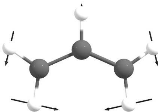
Figure 9.15: Graphical representation of the Q_2 ( A_1 ) normal mode of allyl anion. Obtained at the M06-2X/aug-cc-pVDZ level of theory.
