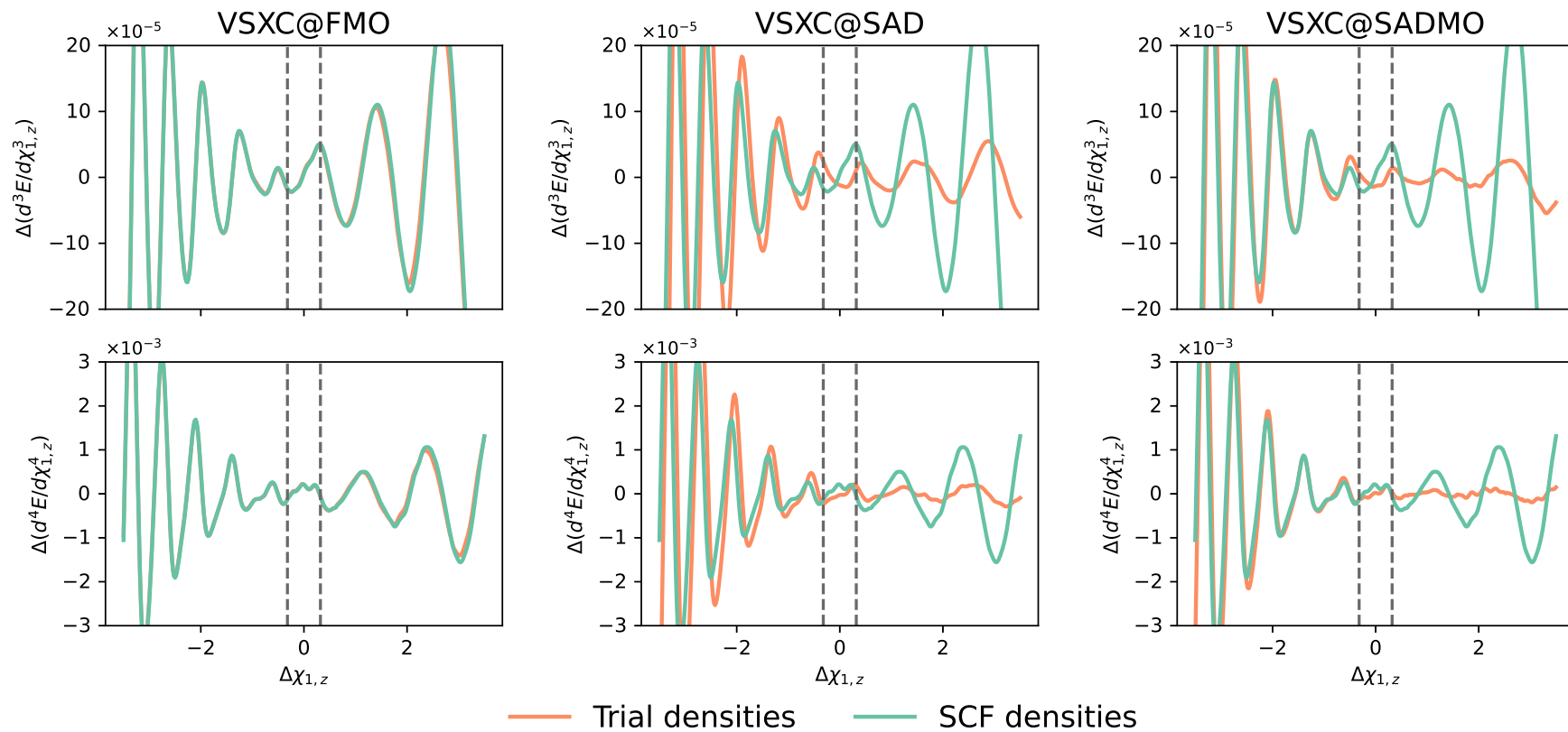
Figure 10.2: Spurious oscillations in d^3E/d\chi_{1,z}^3 and d^4E/d\chi_{1,z}^4 of the \text{HCN} \cdot \text{HF} system, defined as \Delta P = P^{\text{DFA}(99,590)} - P^{\text{DFA}(1500,974)} , obtained with VSXC/6-31+G* and the trial densities (orange curves) and the SCF density (green curves, shown on each plot).
