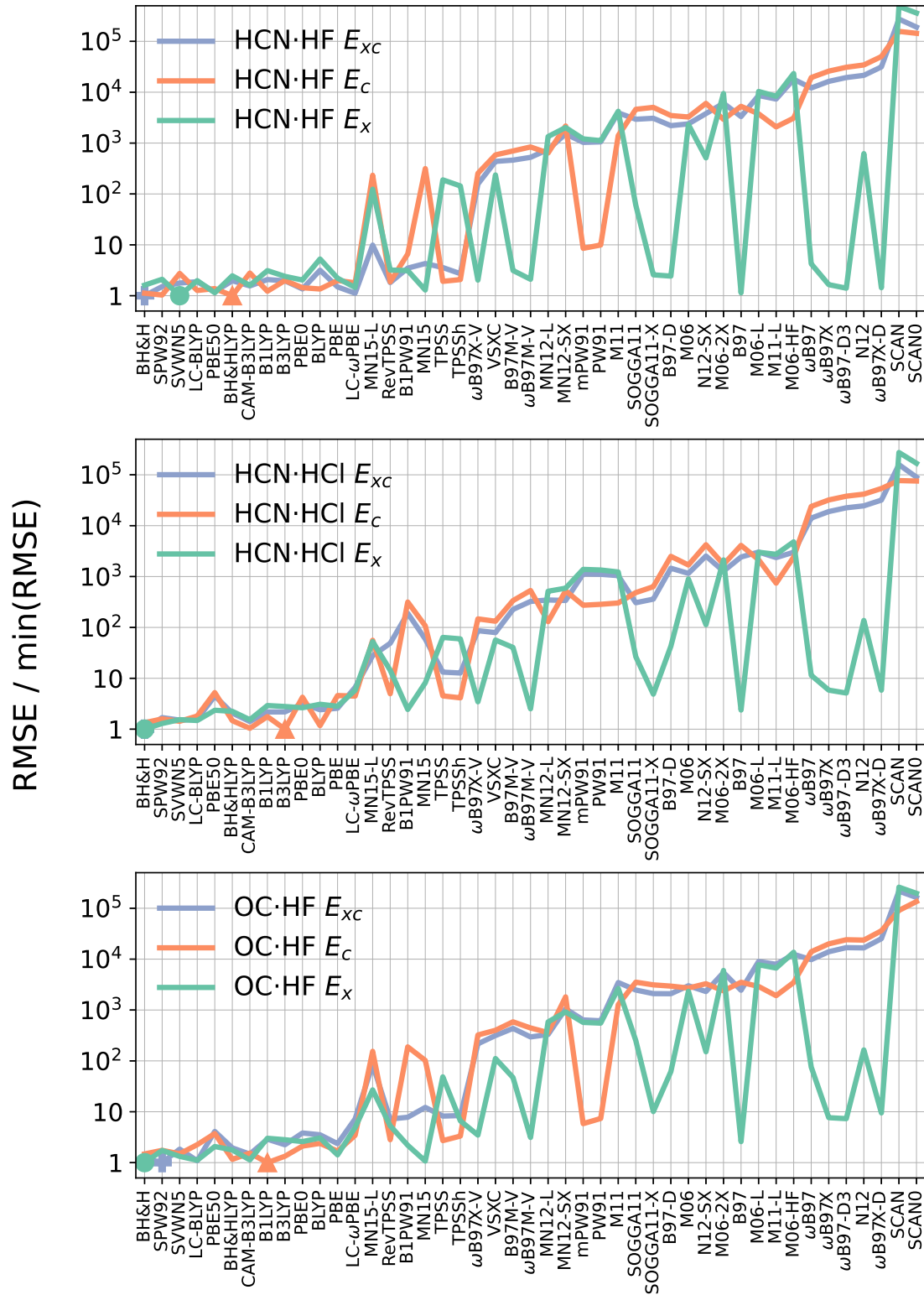
Figure 10.9: The relative values of RMSE in d^4E_{xc}/d\xi^4 , d^4E_x/d\xi^4 , and d^4E_c/d\xi^4 for the HCN·HF, HCN·HCl, and OC·HF, with respect to the minimal RMSE value found within the whole set. The minimum values are marked with a + sign for d^4E_{xc}/d\xi^4 , ▲ for d^4E_c/d\xi^4 , and ● for d^4E_x/d\xi^4 . The ordering of DFAs corresponds to the one in Table 10.2. Results obtained using the (250, 974) grid.
