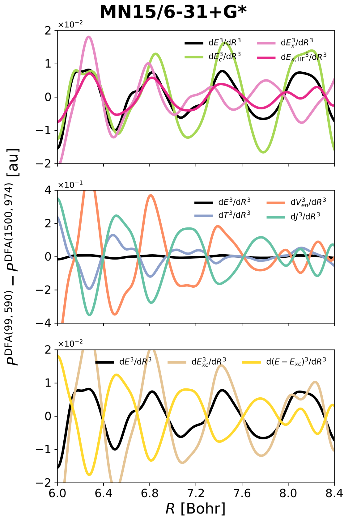
Figure A2.14: Grid-related spurious oscillations in the third derivatives of energy components of Ar_2 : total electronic ( E ), kinetic ( T ), nuclei attraction ( V_{en} ), Coulomb repulsion ( J ), exact HF-like exchange E_{x,HF} , exchange ( E_x ), and correlation ( E_c ), as well as their sums. Obtained with MN15/6-31+G* as the difference between (99, 590) and (1500, 974) integration grids.
