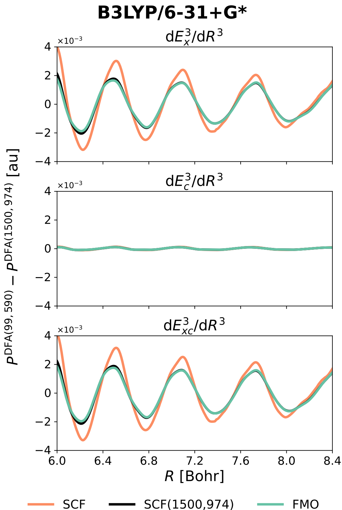
Figure A2.15: Grid-related spurious oscillations in the third derivatives of exchange ( E_x ), correlation ( E_c ) energy components of \text{Ar}_2 , as well as their sum, obtained using B3LYP/6-31+G* and the (99, 590) and (1500, 974) integration grids. Three different types of the input densities are employed: SCF — density obtained in SCF using corresponding grids, SCF(1500, 974) — density obtained in SCF using the reference (1500, 974) grid, FMO — trial density constructed using FMOs obtained for one geometry ( R=7.2 Bohr) and the (250, 974) integration grid.
