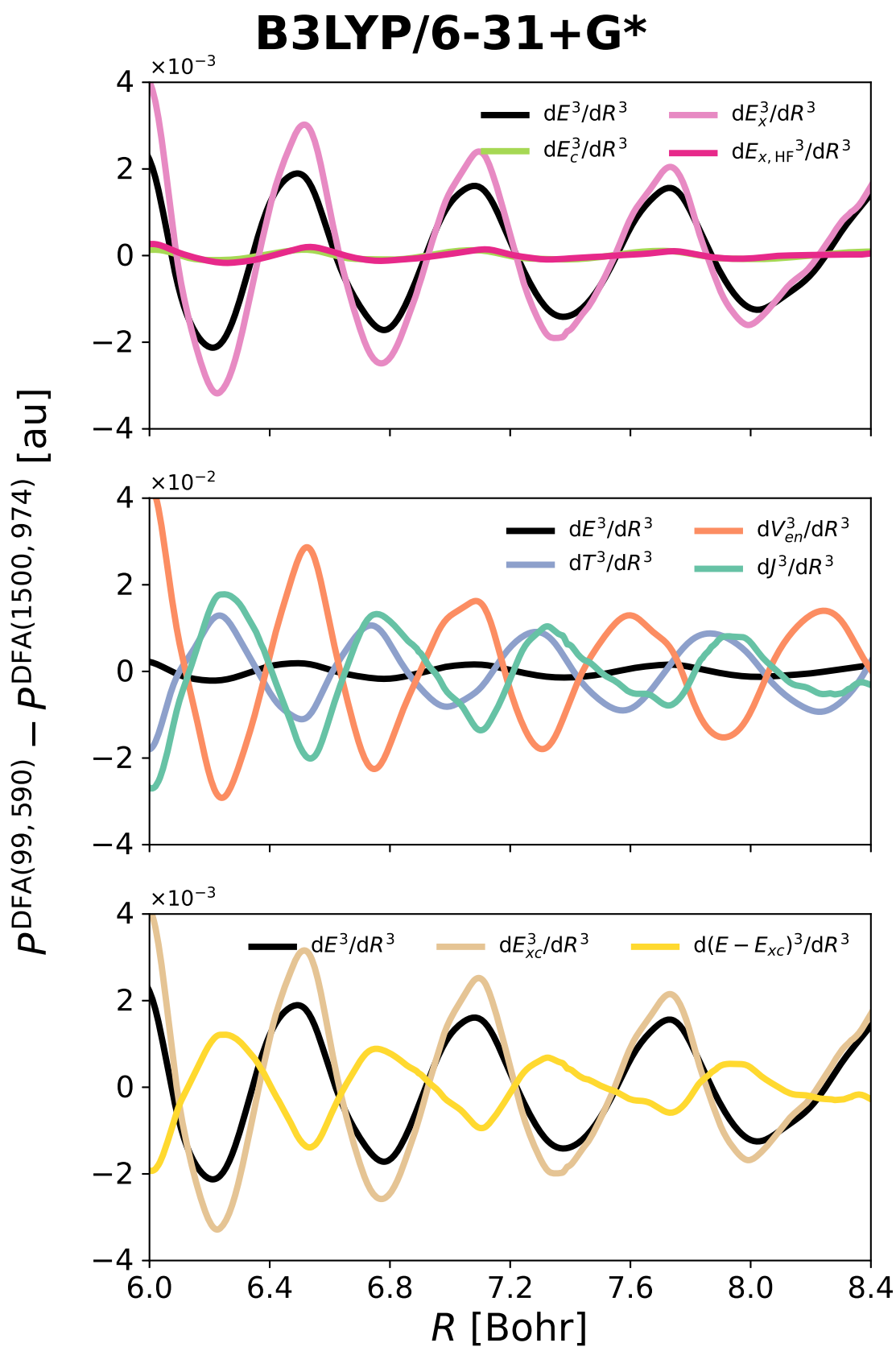
Figure A2.11: Grid-related spurious oscillations in the third derivatives of energy components of \text{Ar}_2 : total electronic ( E ), kinetic ( T ), nuclei attraction ( V_{en} ), Coulomb repulsion ( J ), exact HF-like exchange E_{x,\text{HF}} , exchange ( E_x ), and correlation ( E_c ), as well as their sums. Obtained with B3LYP/6-31+G* as the difference between (99, 590) and (1500, 974) integration grids.
