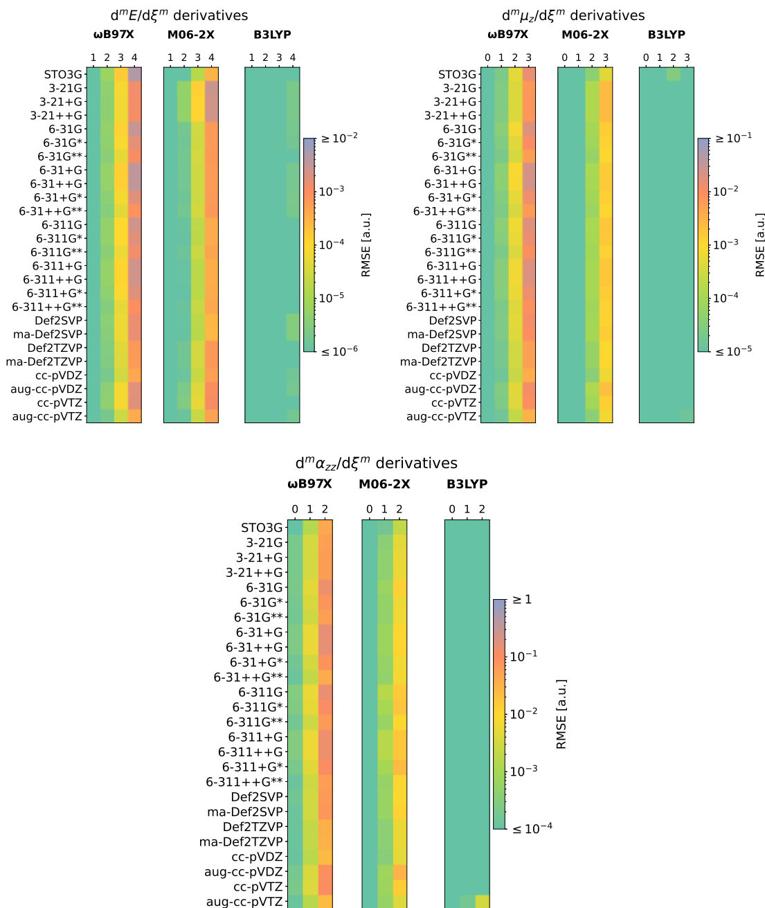
Figure A2.3: Basis set dependence of the grid-related errors in the d^m E / d\xi^m derivatives (left panel, m = 1 - 4 , stored column-wise), the d^m \mu_z / d\xi^m derivatives (middle panel, m = 0 - 3 , stored column-wise), and the d^m \alpha_{zz} / d\xi^m derivatives (right panel, m = 0 - 2 , stored column-wise). Shown for the HCN·HF system and the \omega B97X, M06-2X, and B3LYP functionals combined with the (250, 974) integration grid. Colors reflect the values of the errors in the property measured using RMSE (note the logarithmic scale). Raw data compiled in Tables A3.1 to A3.6.
