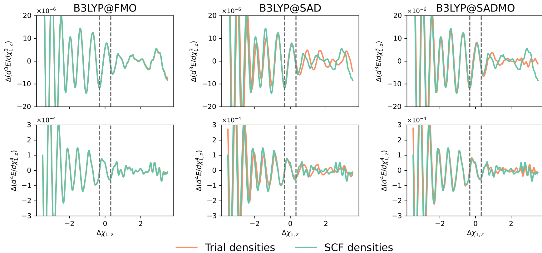
Figure A2.5: Spurious oscillations in d^3E/d\chi_{1,z}^3 and d^4E/d\chi_{1,z}^4 of the \text{HCN} \cdot \text{HF} system, defined as \Delta P = P^{\text{DFA}(99,590)} - P^{\text{DFA}(1500,974)} , obtained with B3LYP/6-31+G* and the trial densities (orange curves) and the SCF density (green curves, shown on each plot).
