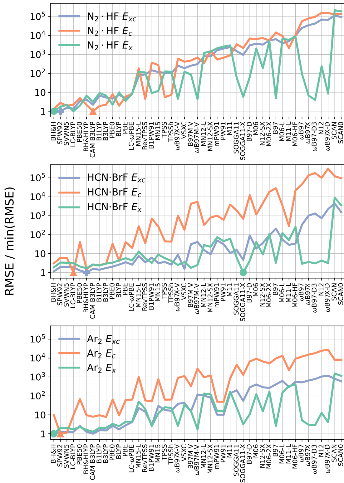
Figure 10.10: The relative values of RMSE in d^4 E_{xc}/d\xi^4 , d^4 E_x/d\xi^4 , and d^4 E_c/d\xi^4 for the N_2 \cdot HF , HCN \cdot BrF , and Ar_2 , with respect to the minimal RMSE value found within the whole set. The minimum values are marked with a + sign for d^4 E_{xc}/d\xi^4 , ▲ for d^4 E_c/d\xi^4 , and ● for d^4 E_x/d\xi^4 . The ordering of DFAs corresponds to the one in Table 10.2. Results obtained using the (250, 974) grid.
