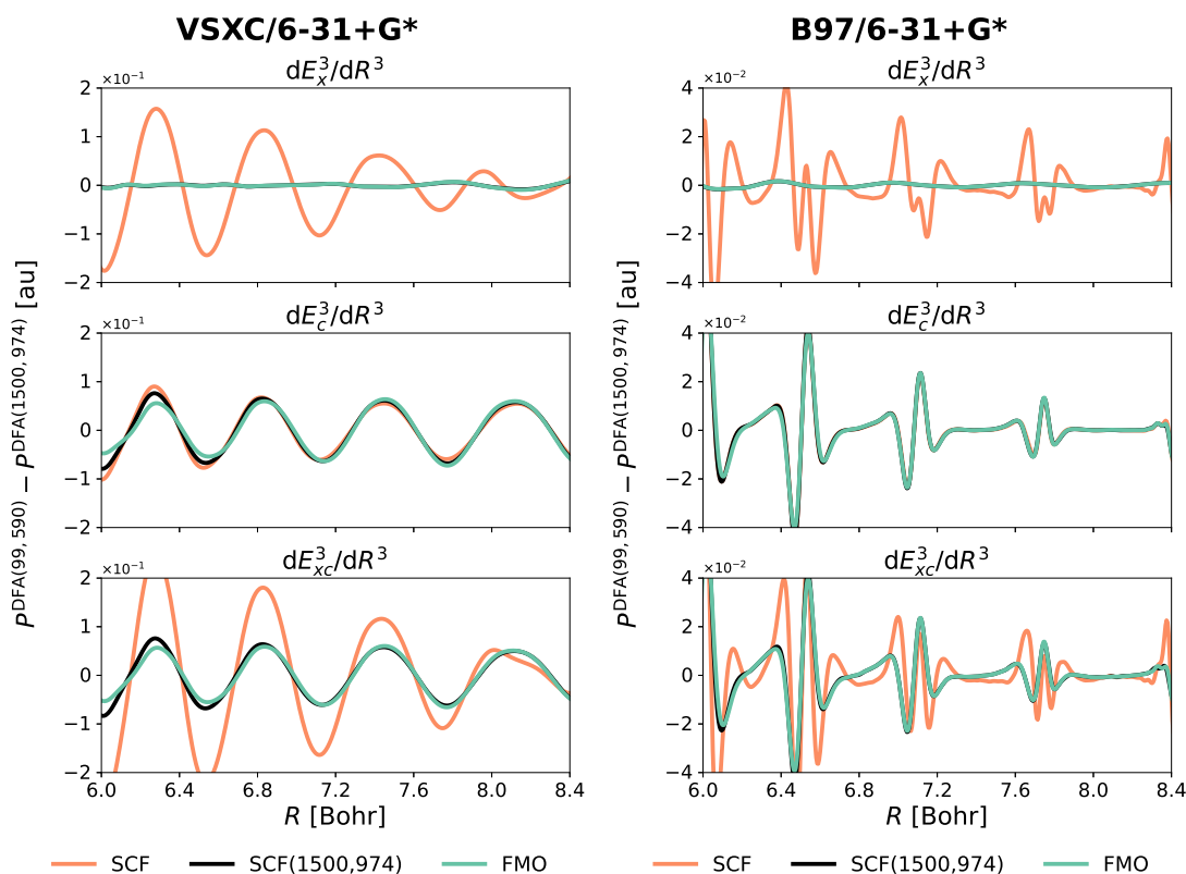
Figure 10.8: Grid-related spurious oscillations in the third derivatives of exchange ( E_x ), correlation ( E_c ) energy components of \text{Ar}_2 , as well as their sum, obtained using VSXC/6-31+G* (left panel) and B97/6-31+G* (right panel), and the (99, 590) and (1500, 974) integration grids. Three different types of the input densities are employed: SCF — density obtained in SCF using corresponding grids, SCF(1500, 974) — density obtained in SCF using the reference (1500, 974) grid, FMO — trial density constructed using FMOs obtained for one geometry ( R=7.2 Bohr) and the (250, 974) integration grid.
