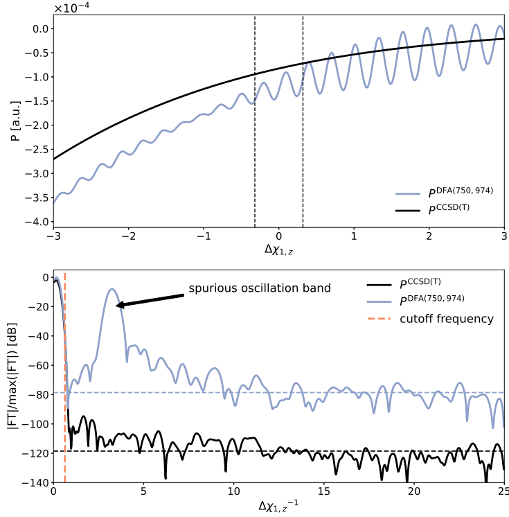
Figure 9.7: Top: d^3E/d\chi_{1,z}^3 curves for HCN·BrH along the \Delta\chi_{1,z} displacement, obtained with the \omega B97X/aug-cc-pVTZ combined with the (750, 974) grid, P^{\text{DFA(LG)}} = P^{\text{DFA(750,974)}} (blue). Property curve obtained with CCSD(T), P^{\text{ref}} = P^{\text{CCSD(T)}} , is shown in black. Bottom: Frequency spectra of P^{\text{DFA(750,974)}} and P^{\text{CCSD(T)}} . The vertical dashed line marks the cutoff frequency for the low-pass filtering of P^{\text{DFA(750,974)}} . The horizontal dashed line marks the noise level in the P^{\text{DFA(750,974)}} and P^{\text{CCSD(T)}} spectra. The band corresponding to the spurious oscillation present in P^{\text{DFA(750,974)}} , is indicated with a black arrow.
