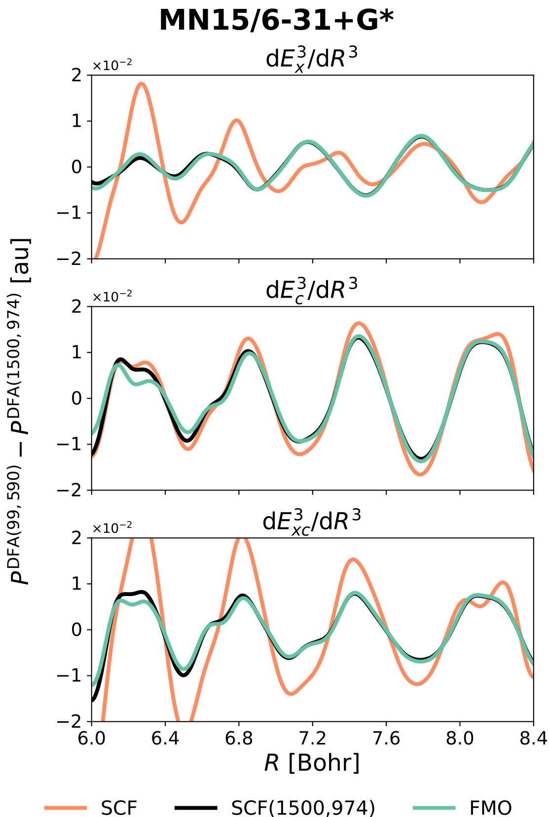
Figure A2.18: Grid-related spurious oscillations in the third derivatives of exchange ( E_x ), correlation ( E_c ) energy components of \text{Ar}_2 , as well as their sum, obtained using MN15/6-31+G* and the (99, 590) and (1500, 974) integration grids. Three different types of the input densities are employed: SCF — density obtained in SCF using corresponding grids, SCF(1500, 974) — density obtained in SCF using the reference (1500, 974) grid, FMO — trial density constructed using FMOs obtained for one geometry ( R=7.2 Bohr) and the (250, 974) integration grid.
