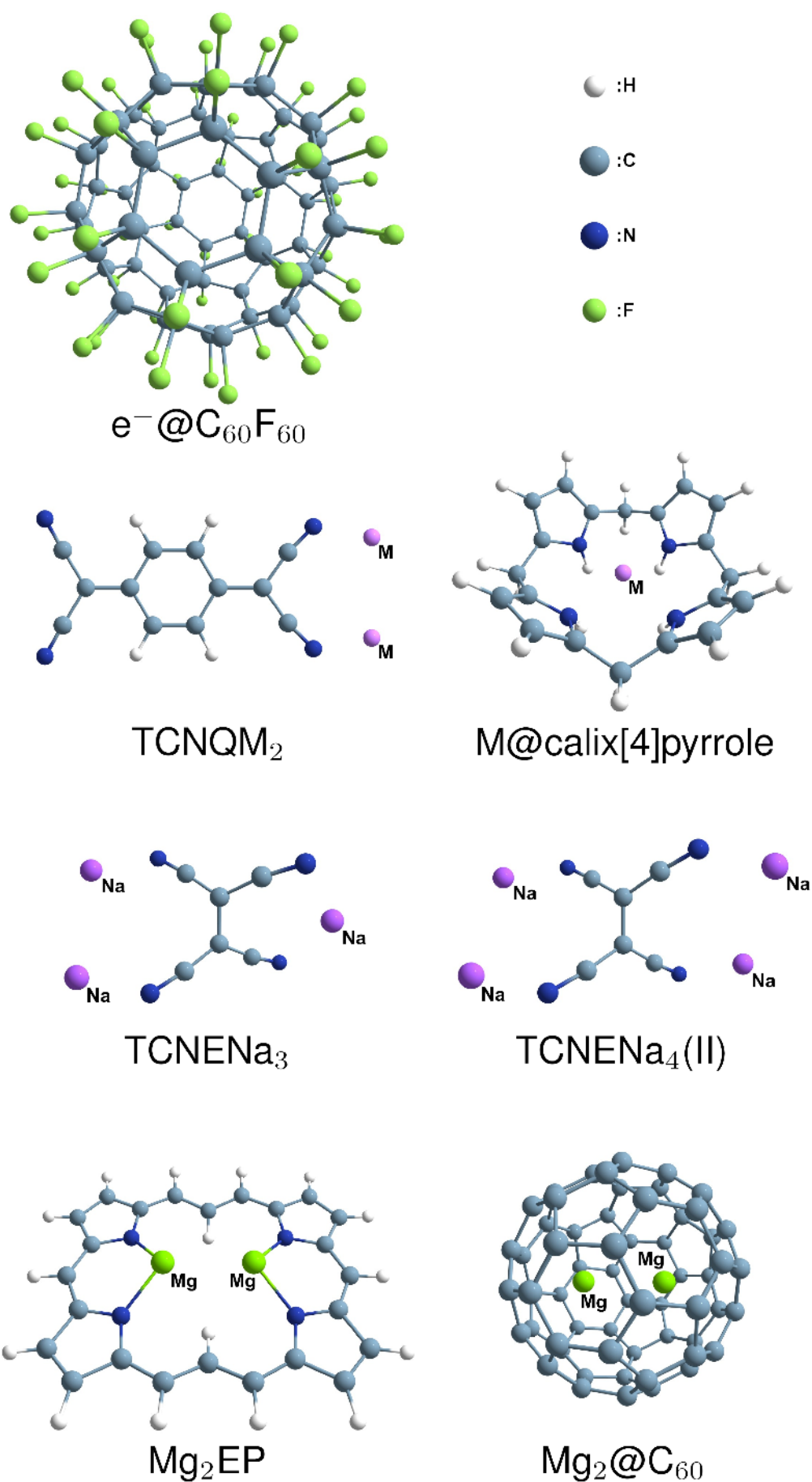
Figure 11.1: From top-left to bottom-right, the molecular structures of e@C_{60}F_{60} , TCNQM_2 , M@calix[4]pyrrole , TCNENa_3 , TCNENa_4(II) , Mg_2EP , and Mg_2@C_{60} , where M atom denotes either M = Li or M = Na.
