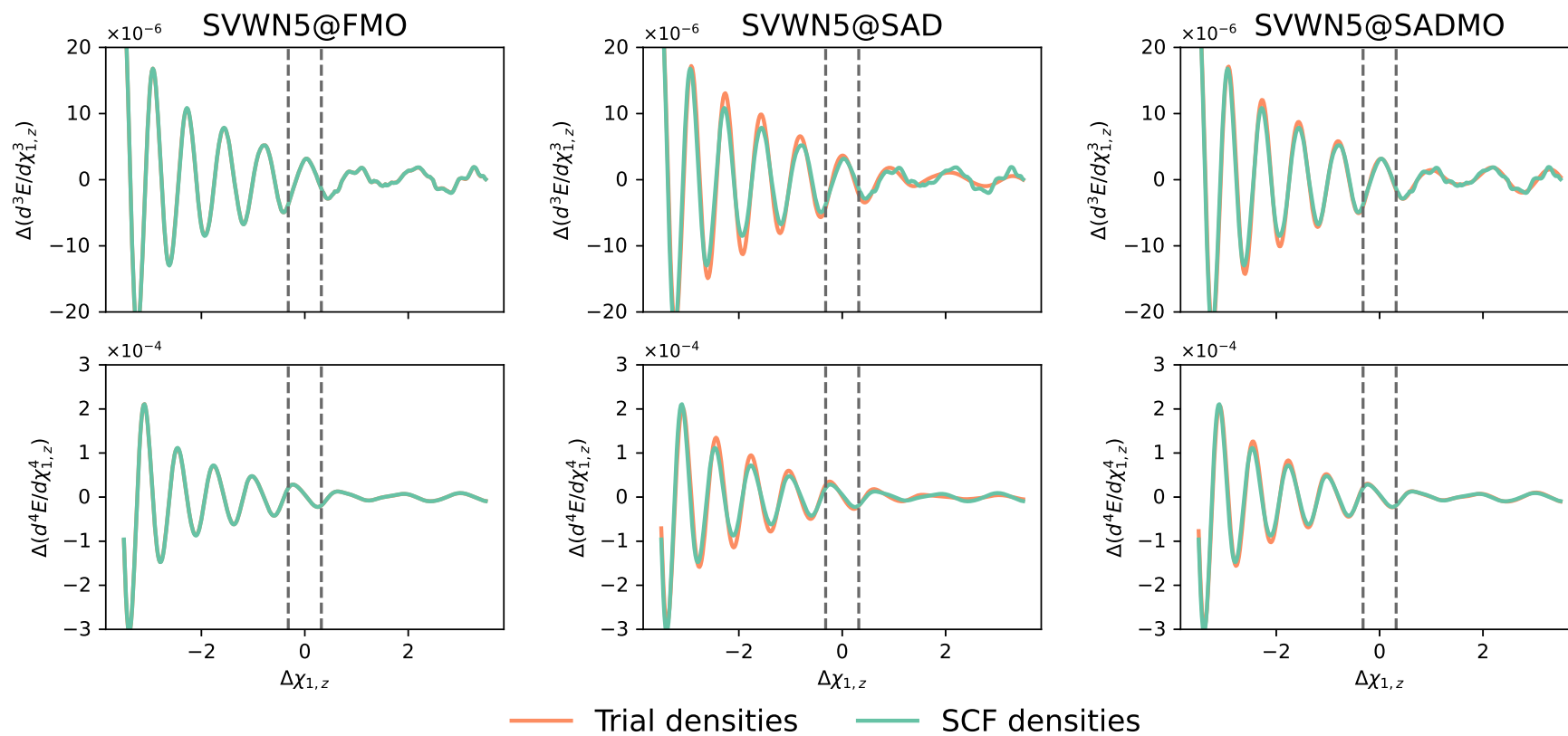
Figure A2.4: Spurious oscillations in d^3E/d\chi_{1,z}^3 and d^4E/d\chi_{1,z}^4 of the HCN·HF system, defined as \Delta P = P^{\text{DFA}(99,590)} - P^{\text{DFA}(1500,974)} , obtained with SVWN5/6-31+G* and the trial densities (orange curves) and the SCF density (green curves, shown on each plot).
