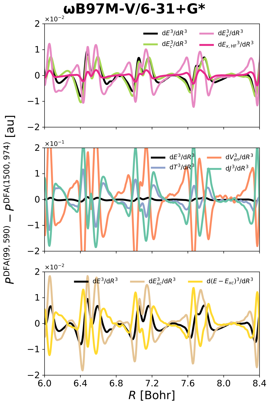
Figure A2.12: Grid-related spurious oscillations in the third derivatives of energy components of \text{Ar}_2 : total electronic ( E ), kinetic ( T ), nuclei attraction ( V_{en} ), Coulomb repulsion ( J ), exact HF-like exchange E_{x,\text{HF}} , exchange ( E_x ), and correlation ( E_c ), as well as their sums. Obtained with \omega B97M-V/6-31+G* as the difference between (99, 590) and (1500, 974) integration grids.
