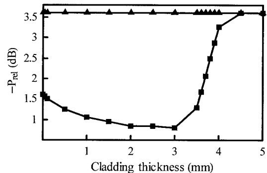
Fig. 8. Simulated values of the relative output power for different cladding thicknesses when the fiber is covered by air (squares) and by oil (triangles). As the cladding thickness increases, the curve corresponding to the air-covered POF converges to the straight line that corresponds to the fiber dipped in oil (congruent to the infinite cladding thickness).
