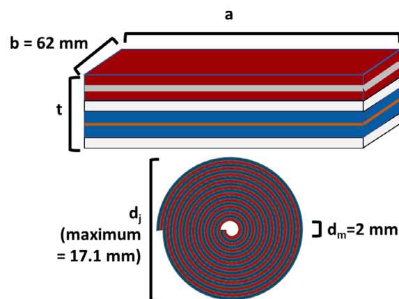
Figure 6. Schematic of jelly roll: unwinded (top) and winded (bottom); total thickness is mentioned as the sum of the thickness of each component of the stack. The dimensions, along with the density of each component, can be used to determine the final weight of the cell (color codes are the same as in Figure 2).
