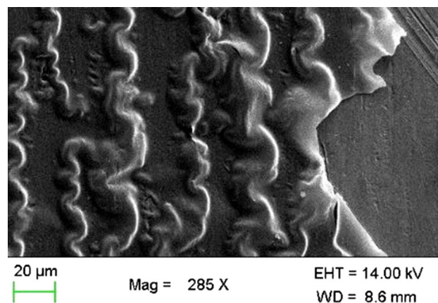
Fig. 12 Deposits collected on the tantalum plate inside the dilatometry chamber after testing Alloy 2 at 1050 °C with a cooling rate of 0.01 °C/s
