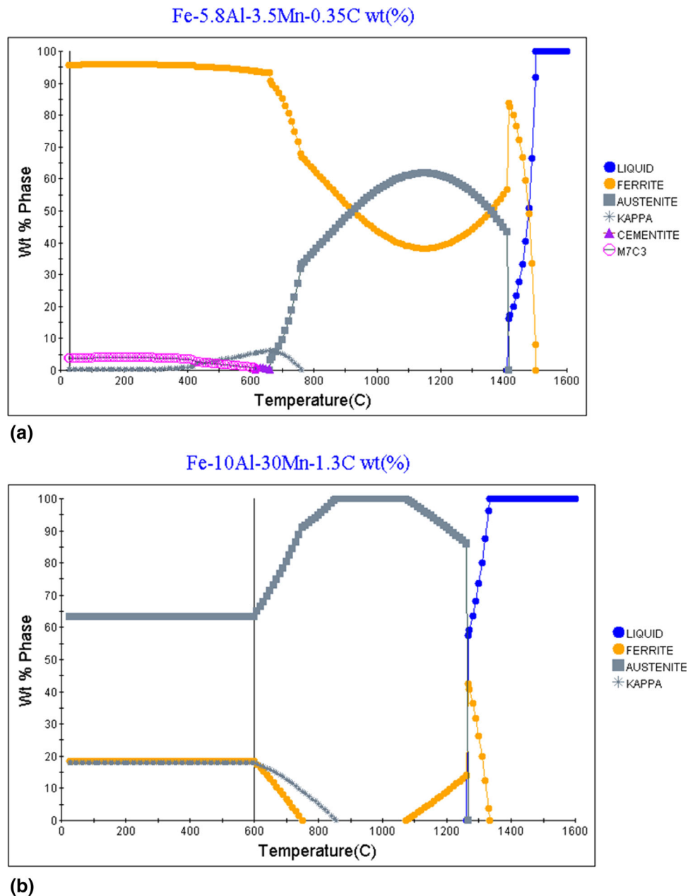
Fig. 4 Phases present at different temperatures obtained with JMatPro for Alloy 1 (a) and Alloy 2 (b)
