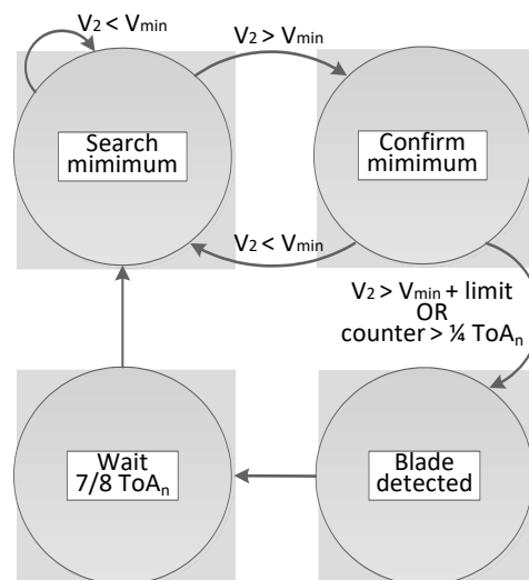
Figure 7. Pseudo-state machine to detect global minima.
